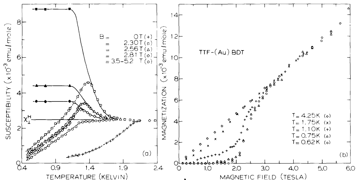
Fig. 5. Susceptibility vs. temperature (a) and magnetization vs. field (b) for TTF-AuBDT. Data for B = 0 (a) and T = 1.10, 1.75 and 4.25 K (b) are from ref. [3]. ( \chi_H^1 is the theoretical susceptibility for the uniform antiferromagnetic Heisenberg chain.) In (a) closed symbols represent the static \chi whereas open symbols refer to the differential \chi for \nu = 18-1880 Hz.
