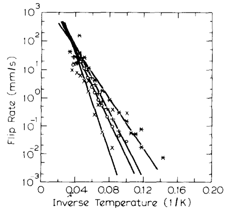
Fig. 13. The flip rate of the BT fits to the spectra of \text{RbFeCl}_3 \cdot 2\text{H}_2\text{O} obtained with an applied field of 1.5 (*) , 2.25 (+), 3.0 ( \circ ), and 6.0 ( \times ) Tesla along the c -axis. The solid lines illustrate the activated processes.
