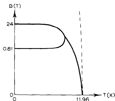
Fig. 4. A schematic representation of the phase diagram for \text{RbFeCl}_3 \cdot 2\text{H}_2\text{O} , drawn after ref. [21]. The solid and the broken lines represent the phase boundaries if the applied field is parallel to the ferro- and antiferromagnetically aligned spin components, respectively.
