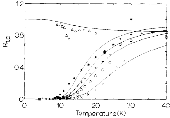
Fig. 11. Ratio of transition probabilities, R_{tp} , of \text{RbFeCl}_3 \cdot 2\text{H}_2\text{O} versus temperature for B_a = 3 \text{ T} ( \Delta ) and B_c = 1.5, 2.25, 3.0, 6.0 \text{ T} (*, +, \circ , \times , respectively). The solid lines represent the predictions for an ideal S = 1/2 Ising chain.
