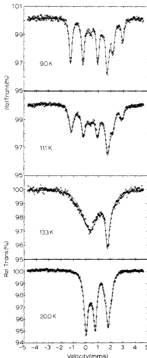
Fig. 10. Representative single crystal spectra of \text{RbFeCl}_3 \cdot 2\text{H}_2\text{O} measured in a field of 3 T along the a axis. The solid lines represent the fit using the Blume and Tjon model.
