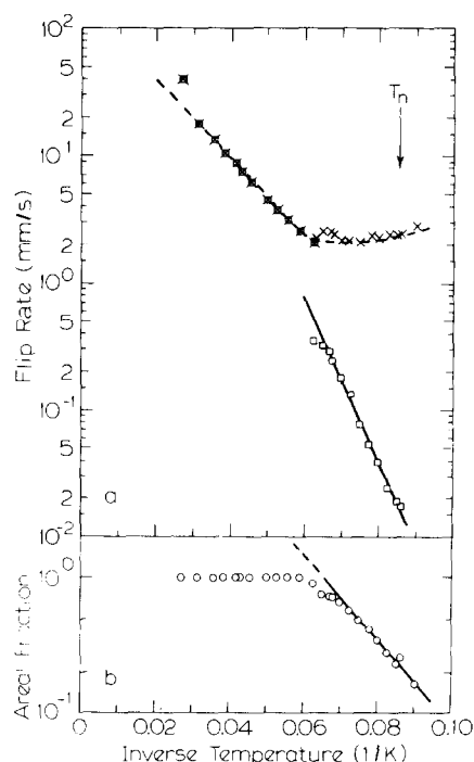
Fig. 8. The flip rate of the slowly ( \square ) and fast ( \times ) relaxing subspectra of \text{FeC}_2\text{O}_4 \cdot 2\text{H}_2\text{O} . The lower part shows the relative intensity of the fast relaxing component. The solid lines illustrate the activated processes.
