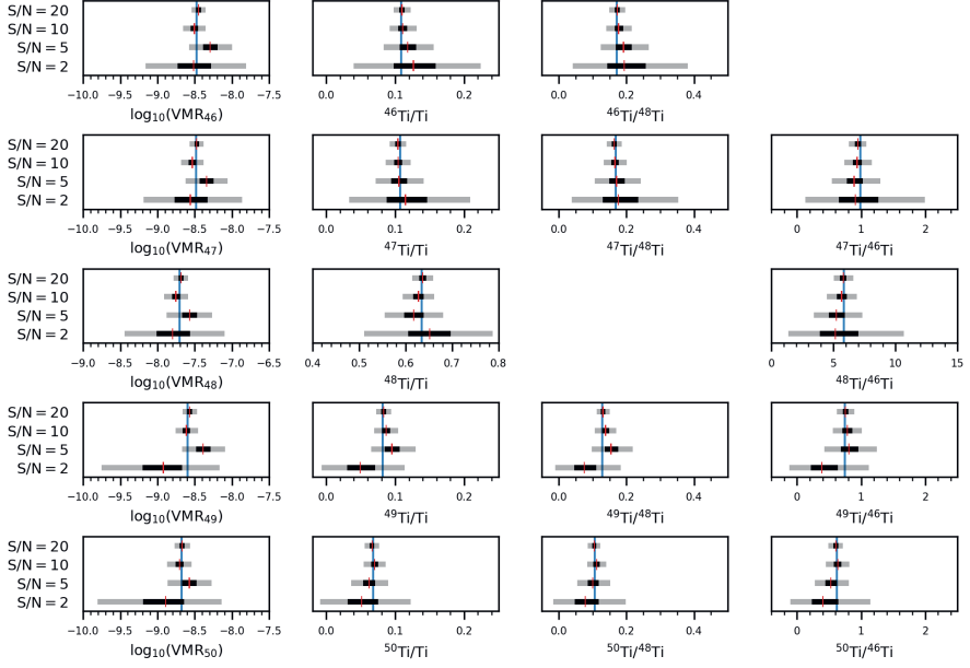
Figure 3.3. Same as Figure 3.2, but for the MCMC retrievals of TiO features in the narrow, broadband-filtered CARMENES spectrum of GJ 1002 with various levels of noise added. The results from the retrieval of the narrow, broadband-filtered spectrum without added noise are shown by the vertical blue lines.
