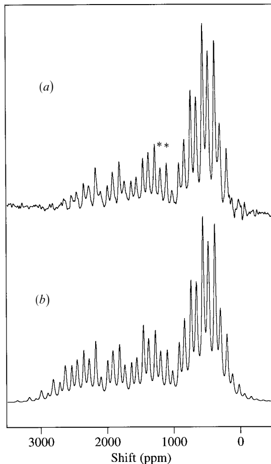
Figure 2. (a) MAS NMR Spectrum of 13 C-2 DMTM(TCNQ) 2 at 300 K. The isotropic shifts are illustrated with asterisks and are referenced to TMS. The spinning speed was \omega_r/2\pi = 18\,000 kHz, 50 000 scans were added with a recycle time of 30 ms. (b) A simulation using parameters derived from the best fit to the derivative of the spectrum in (a); \delta_{\text{iso,I}} = 1094 ppm, \delta_{11,\text{I}} = 244 ppm, \delta_{22,\text{I}} = 269 ppm, \delta_{33,\text{I}} = 2770 ppm, \delta_{\text{iso,II}} = 1193 ppm, \delta_{11,\text{II}} = 274 ppm, \delta_{22,\text{II}} = 275 ppm, \delta_{33,\text{II}} = 3031 ppm.
