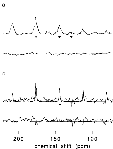
FIG. 2. ^{13}\text{C} MAS spectrum (a) and difference spectrum (b) for [5\text{-}^{13}\text{C}] retinal-labeled bacteriorhodopsin under heteronuclear (CW) decoupling at spinning speed \omega_r/2\pi = 2.5 kHz. The centerbands of the label (144.3 ppm), the natural-abundance carbonyl (176 ppm), and the natural-abundance aromatic carbons (129 ppm) are marked with an asterisk. The results of the analyses are represented by the smooth line in the spectra. Below each spectrum the residues, data minus fit, are shown.
