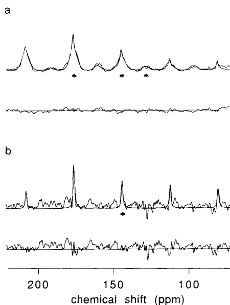
FIG. 2. ^{13}\text{C} MAS spectrum (a) and difference spectrum (b) for [5- ^{13}\text{C} ]retinal-labeled bacteriorhodopsin under heteronuclear (CW) decoupling at spinning speed \omega_r/2\pi = 2.5 kHz. The centerbands of the label (144.3 ppm), the natural-abundance carbonyl (176 ppm), and the natural-abundance aromatic carbons (129 ppm) are marked with an asterisk. The results of the analyses are represented by the smooth line in the spectra. Below each spectrum the residues, data minus fit, are shown.
