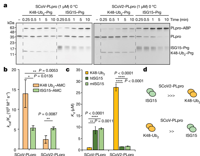
Fig. 1 | DeISGylating and deubiquitylating activities of SCoV-PLpro and SCoV2-PLpro. a , SCoV-PLpro (left) or SCoV2-PLpro (right) were incubated with indicated Prg probes. Experiments were repeated three times independently with similar results. b , Catalytic efficiency ( k_{cat}/K_m ) of SCoV2-PLpro and SCoV-PLpro cleavage of K48-Ub 2 -AMC or ISG15-AMC. c , Dissociation constant ( K_d ) of SCoV2-PLpro and SCoV-PLpro. Data in c , d , are mean \pm s.d. or mean \pm s.e.m. ( n = 3 independent experiments). * P < 0.05 , ** P < 0.01 , **** P < 0.0001 ; two-tailed paired t -test. d , Schematic representation of substrate specificity of SCoV2-PLpro (red) and SCoV-PLpro (blue). The preferred substrate is shown on the left.
