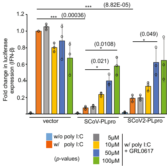
Extended Data Fig. 6 | Effect of PLpro on IFN-β or NF-κB p65 expression level. level. a, b, Effect of PLpro on IFN-β (a) or NF-κB p65 (b) expression level. A549 Cells were transfected with indicated GFP-PLpro and treated with either poly(I:C) or TNF-α to induce IFN-β and NF-κB p65 expression, respectively. c, d, Effect of GRL-0617 on PLpro mediated IFN-β (c) or NF-κB p65 (d) expression
