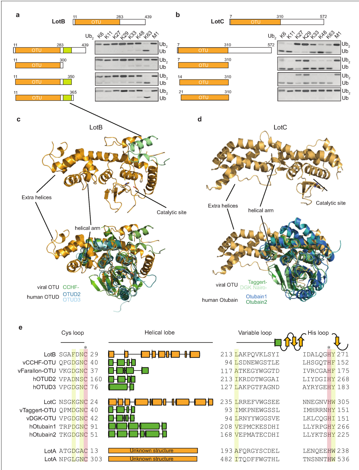
Figure 3. Structural comparison of Legionella OTU-deubiquitinases with other OTU-family. (a, b) Minimal domain boundaries of catalytically active LotB and LotC. Different constructs were cloned based on the predicted OTU-domains and their activity, and were tested with di-Ub panel. (c, d) Structural comparison of LotB and LotC with the closest homologues. CCHF- (PDB: 3PHU), OTUD2 (PDB: 4BOQ), OTUD3 (PDB: 4BOU), Taggart- (PDB: 6D × 3), Figure 3 continued on next page
