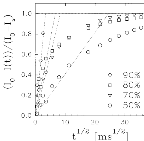
Figure 3. Results of the spin-diffusion measurement as described in the text. The intensity of the narrow fraction of the spectrum after spin diffusion, [I(0) - \{I(t) \exp(t/T_1)\}] / [I(0) - I_s] , is plotted versus the square root of the spin-diffusion period t . In this expression for I(0) and I_s are the intensity at t = 0 and t = \infty , respectively. The exponential factor corrects for the loss of signal due to T_1 spin-lattice relaxation; T_1 is 0.8 s here. The dashed lines cross the saturation level at a time t^* that is used to calculate the characteristic domain size. 8,11
