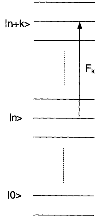
Figure 2. The sample rotation is mapped on a single manifold of Fourier states |n\rangle by the renormalization. The transition operators couple between different states.
