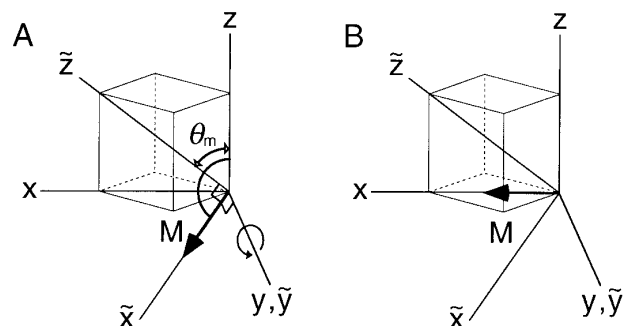
FIG. 2. (A) Starting with a (\pi/2 + \theta_m)_y pulse, the component along the \tilde{z} axis is zero, and (B) any component in the plane perpendicular to the \tilde{z} axis is selected by the \theta_{m,y} back pulse.
