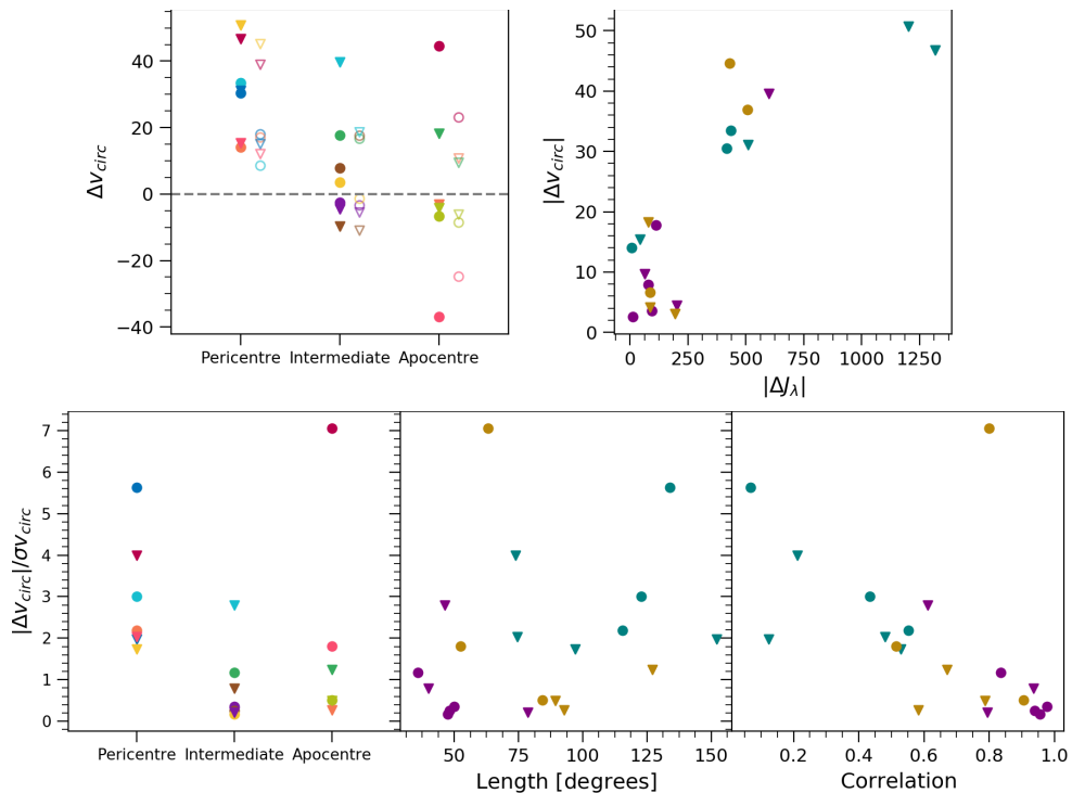
Figure 3.7.1: The residuals of the circular velocity curve at the distance of the smallest 1\sigma uncertainty as a function of the sections’ properties. On the top left panel, we also show the residuals at the sections’ median distance with lighter empty markers, for comparison. On the left panels, we adopt our section-specific colour scheme, while on the rest of the panels we indicate the pericentre, intermediate and apocentre sections with teal, purple and yellow colours, respectively. A description of how the stream properties were computed is available in Appendix 3.B.
