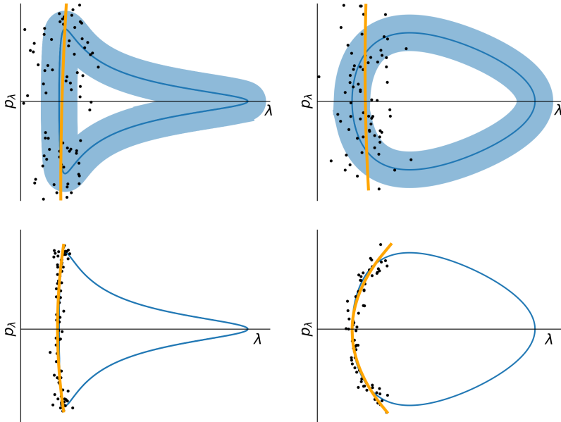
Figure 3.7.2: Schematic phase diagram of dwarf galaxy streams (top panels) and cold stellar streams (bottom panels) near pericentre passage for radial orbits (left panels) and circular orbits (right panel). The black points represent stream stars created by selecting points along the pericentre of the orbit shown with the blue line and adding scatter in both \lambda and p_\lambda . This scatter is 5 times larger in both positions and momenta for the dwarf galaxy streams compared to the cold stellar streams. The light blue shaded regions on top panels approximate the much larger “scatter” in the orbits of dwarf galaxy streams. The yellow lines show a fit to the black points on each panel.
