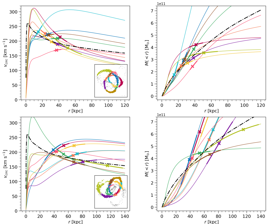
Figure 3.5.1: The best-fit Stäckel potentials for different sections of stream A (top panels) and stream B (bottom panels) shown in circular velocity and enclosed mass profiles. The crosses mark the median distance of each section, while the thicker part of the lines corresponds to the full range of distances of star particles in that section. The insets show the stream in x-z frame for reference.
