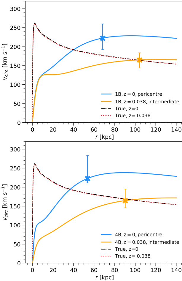
Figure 3.7.3: Comparison of the results from analysis of the present day and past ( z = 0.038 ) positions of the stars in sections 1B (top panel) and 4B (bottom panel). The solid coloured lines represent the best-fit Stäckel potential and the error bar shows the 1\sigma uncertainty at the median galactocentric distance for each data set. The black and red dash-dotted lines represents the true galactic potential at z = 0 and z = 0.038 , respectively.
