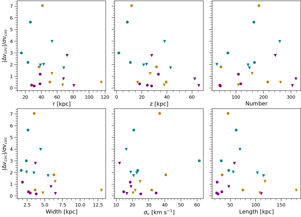
Figure 3.B.1: The residuals of the circular velocity curve at the distance of the smallest 1\sigma uncertainty as a function of the sections' properties. We indicate the pericentre, intermediate and apocentre sections with teal, purple and yellow colours, respectively.
