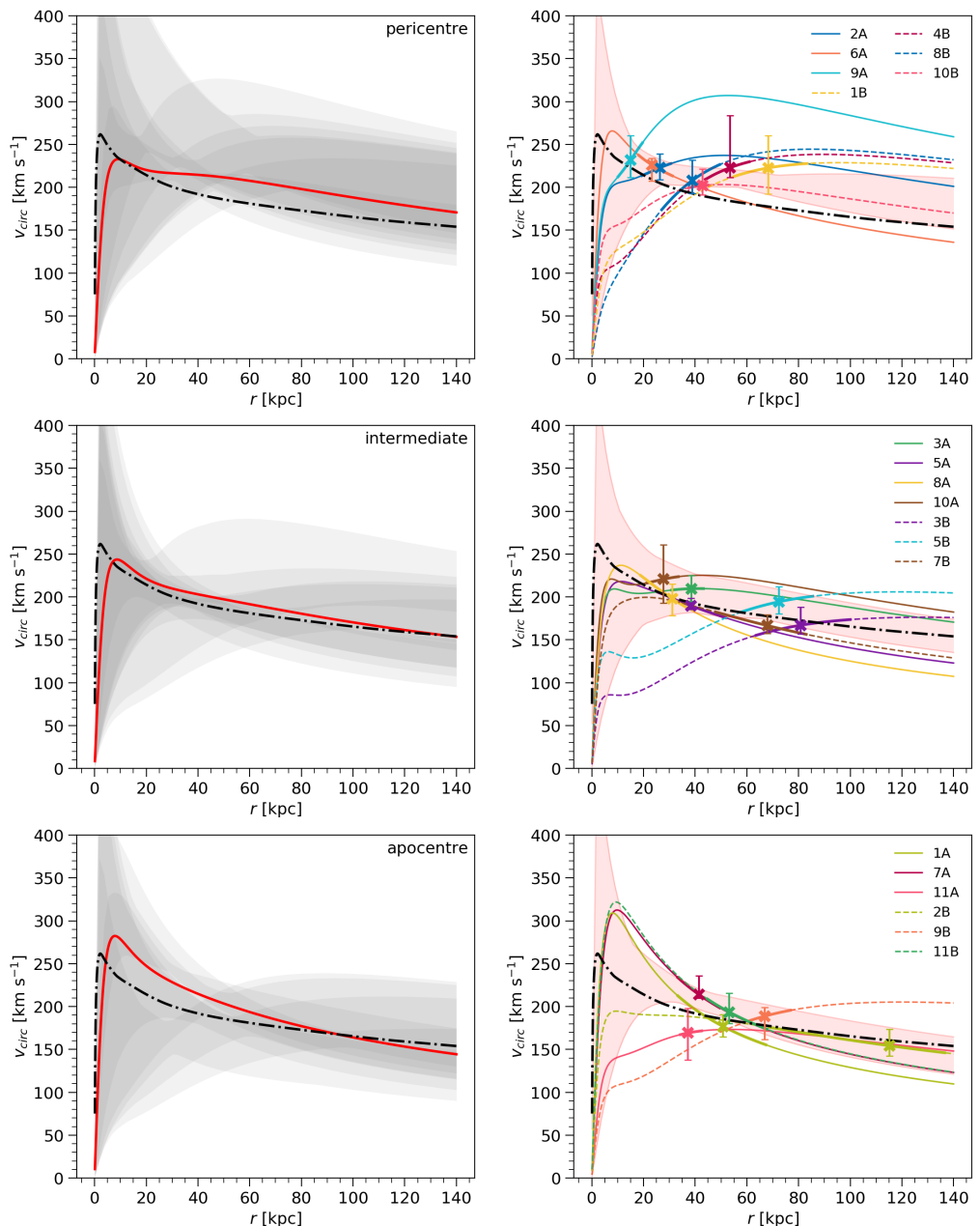
Figure 3.6.1: The results of all stream A and stream B sections organised by orbital phase. The top, middle and bottom panels show the pericentre, intermediate and apocentre sections, respectively. The coloured lines in the right panels show the best-fit Stäckel potential of the individual sections, the error bar indicates the uncertainty at their median distance. The solid and dashed lines correspond to stream A and stream B sections, respectively. The full confidence regions of these results are shown on the left panel as grey semi-opaque regions. The red line in the left panel shows the best-fit Stäckel potential of the joint phase data set, and the red shaded area on the right panel is its associated uncertainty. The true potential is shown with a black dash-dotted line in every panel.
