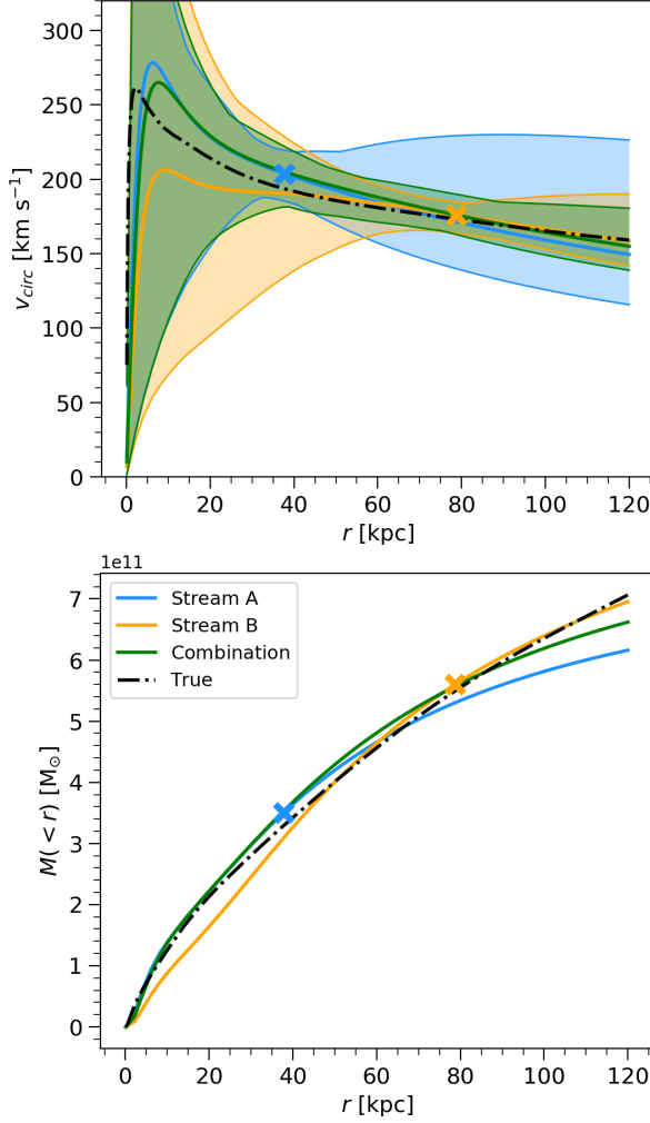
Figure 3.4.1: Results for stream A, stream B and their combined data. We compare the results from these data sets to the true potential (black dash-dot line) in circular velocity and enclosed mass. The solid coloured lines show the best-fit Stäckel potential of each data set and the shaded regions show the corresponding 1\sigma uncertainty regions. The median distance of the star particles in the stream A and stream B data sets are marked with a cross (see Table 3.1).
