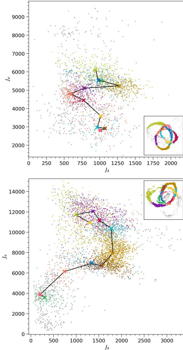
Figure 3.4.4: The action-space of stream A (top) and B (bottom) in their respective best-fit potentials. The insets show the stream in x - z frame for reference. The star particles are coloured based on their sections (see Table 3.1) with star particles not belonging to any section shown as grey. The centre of each section is marked with an “X” in its respective colour, and the black line connects them in the order they appear in phase space.
