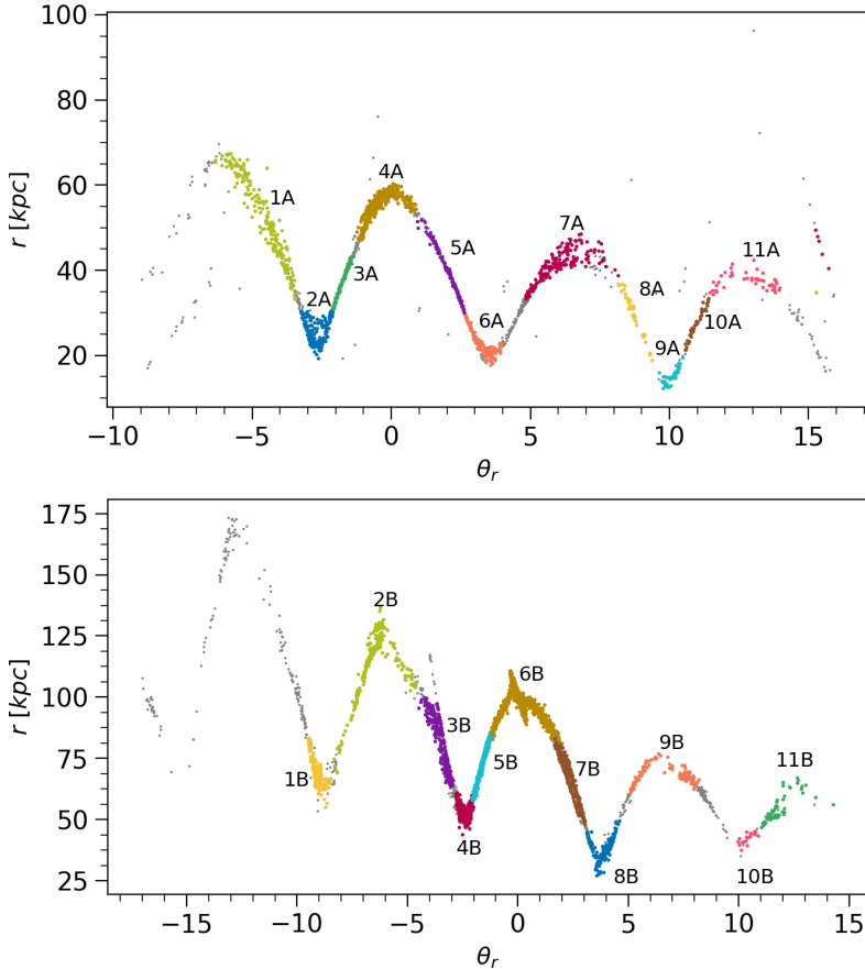
Figure 3.3.1: Phase information of streams A (top) and B (bottom). The progenitor-containing section (in gold) is at \theta_r = 0 . Colour scheme as in Figure 3.2.1 (see also Table 3.1).
