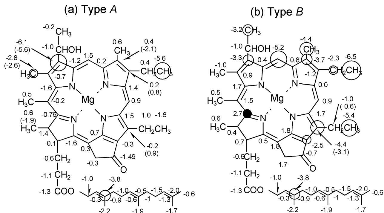
Figure 7. Schematic map showing the ^{13}\text{C} chemical shift difference, \Delta\delta = \delta_{\text{solid}} - \delta_{\text{monomer}} , for the type A (a) and B (b) of (3^1R) -[ E,E ]BChl c_F in the \text{CH}_2\text{Cl}_2 -treated solid aggregate. All values were obtained using Table 1. The ^{13}\text{C} chemical shifts of monomeric (3^1R) -[ E,E ]BChl c_F are collected in a mixture of \text{CDCl}_3 and \text{CD}_3\text{OD} (v/v 1:9). 13 The carbons with the \Delta\delta > \pm 2.0 ppm are marked with a circle in the map. Open and closed circles correspond with negative and positive \Delta\delta , respectively. The sizes of the circles reflect the magnitude of the \Delta\delta .
