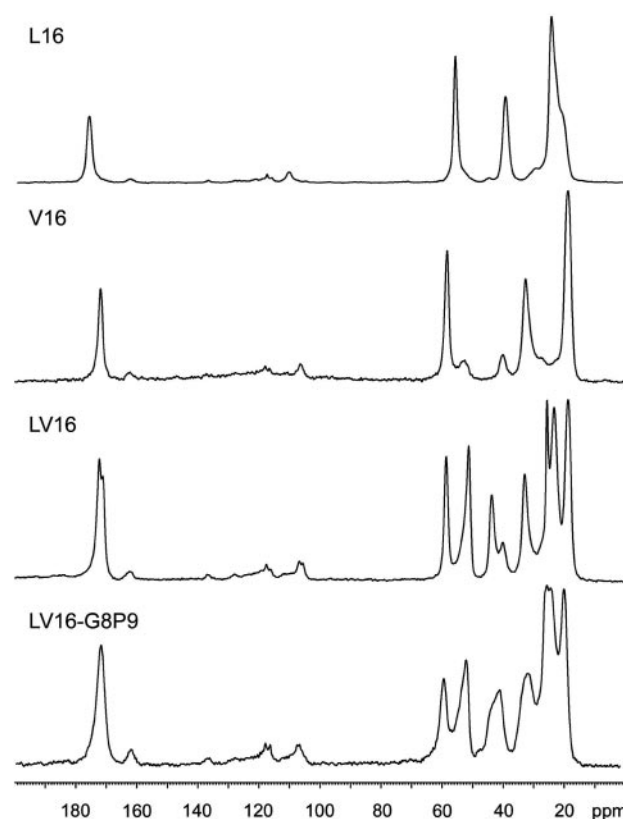
Fig. 6. One-dimensional 13 C-natural abundance CP-MAS solid-state NMR spectra of lyophilized peptides. Please note the different 13 C-carbonyl resonances for L16 and V16. The resonances from 20 ppm to 60 ppm correspond to C \alpha , C \beta , and side-chain carbons.
