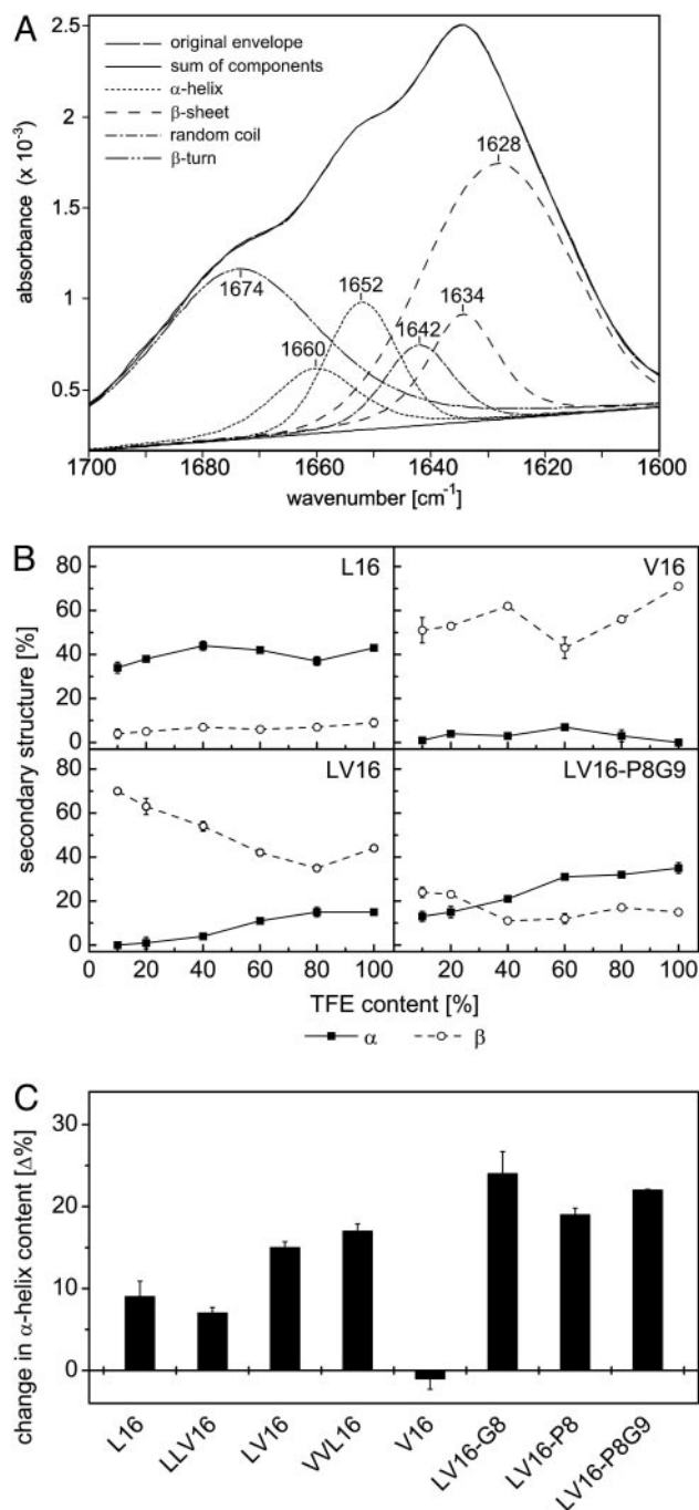
Fig. 5. Structural plasticity of LV peptides determined by FTIR spectroscopy. (A) Original spectrum of LV16 in 100% TFE and decomposition of the amide-I band into individual bands according to ref. 27; the superposition of the original envelope with the sum of components demonstrates the quality of the fit. (B) \alpha -Helix and \beta -sheet contents of some peptides (1.5 mg/ml) upon titration from TFE solution. (C) Conformational change of peptides as revealed by differences in helix content seen at 10% and 100% TFE, respectively. Gains in secondary structure upon decreasing polarity result in positive values. Note that the changes in helix contents tended to be larger with the more fusogenic peptides. Data are shown as means \pm SE ( n = 3 ); error bars were omitted when they were smaller than the symbols. Results obtained with peptide LV16-G8P9 are not shown because it adhered to the cuvette surface with unknown effects on its secondary structure.
