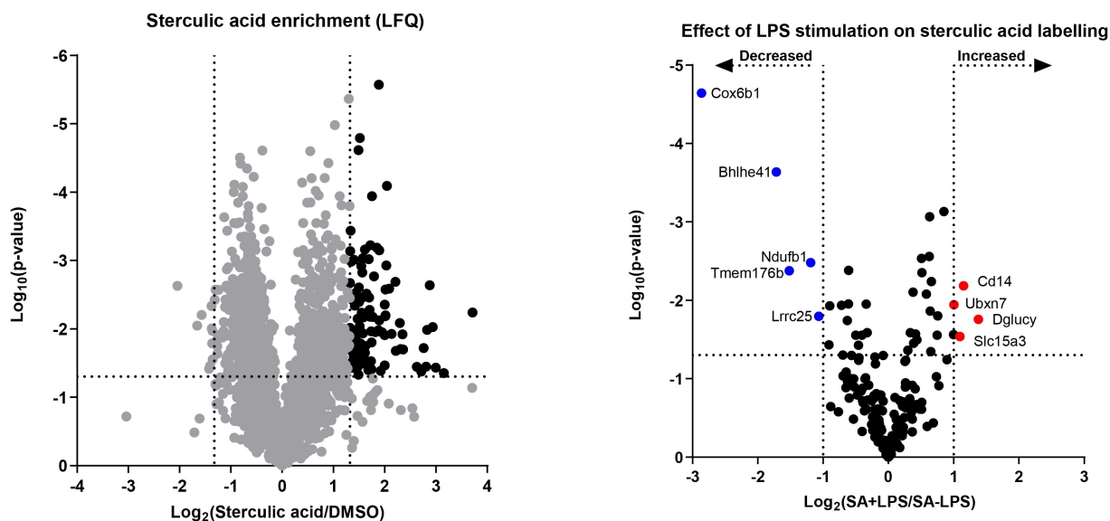
Figure 5. Proteomic analysis of proteins modified with 1 in DC2.4 cells by chemical proteomics. DC2.4 cells were stimulated with or without LPS ( 100 \text{ ng mL}^{-1} ) for 24 h and treated with 1 ( 10 \mu\text{M} ) for 20 h. Left: Volcano plot of proteins identified in pulldown experiment with 1 ( 10 \mu\text{M} ) and biotin-PEG4-tetrazine ( 200 \mu\text{M} ). Proteins with a ratio > 2.5 and p\text{-value} < 0.05 are considered specifically enriched and are highlighted in black. Right: Difference in steric acid-labeling of proteins between LPS- or vehicle-treated DC2.4 cells. LFQ-values of specifically steric acid-enriched proteins were compared and proteins with significantly higher LFQ abundance between the two conditions are marked in red and blue for LPS- and vehicle-treated conditions, respectively.
