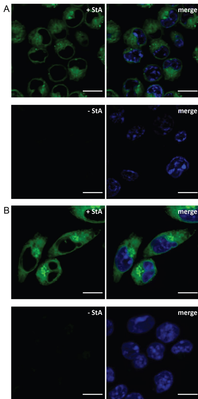
Figure 3. Confocal imaging of DC2.4 cells incubated with 1 (+ StA, 50 μM) or without the probe (-StA). A) Live-cell imaging of labelled cells visualised with 19 (5 μM). B) Fixed-cell imaging of labelled cells visualised with 8 (5 μM). The samples were washed after metabolic incorporation of 1 and after ligation with the fluorophore-tetrazines, and were imaged at > 4 distinct locations in the same well. DNA was counterstained with Hoechst 33342 (blue) for reference. Scale bars represent 10 μm.
