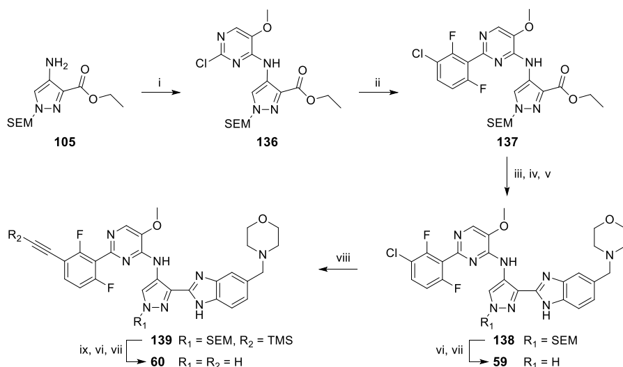
Scheme 4.6 | Synthesis of 59 and 60. Reagents and conditions: i) 2,4-dichloro-5-methoxypyrimidine, DIPEA, EtOH, 50°C, 78%. ii) (3-chloro-2,6-difluorophenyl)boronic acid, K 2 CO 3 , XPhos Pd G2, THF/H 2 O (1:2). iii) LiOH, MeOH/H 2 O (1:1), DCM, 65°C. iv) 4-(morpholinomethyl)benzene-1,2-diamine (synthesized in Chapter 2 , compound 28), EDC-HCl, HOBT, DMF. v) AcOH, 118°C, 9% over two steps. vi) TFA, DCM. vii) ethylenediamine, DCM/MeOH (1:1), 88 – 95%. viii) trimethyl((tributylstannyl)ethynyl)silane, XPhos, Pd 2 (dba) 3 , THF, 135°C (sealed tube), quant. ix) TBAF, THF.
