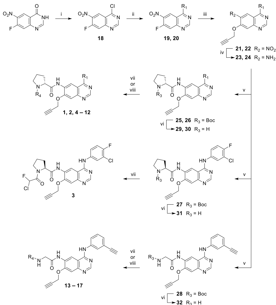
Scheme 5.1 | Synthesis of 1 – 17. Reagents and conditions: i ) \text{SOCl}_2 , cat. DMF, 75^\circ\text{C} , 99%. ii ) 3-chloro-4-fluoroaniline (for 19 ) or 3-ethynylaniline (for 20 ), DIPEA, 2-propanol, 37 – 81%. iii ) propargyl alcohol, \text{KOtBu} , THF, 0^\circ\text{C} – RT, 91% – quant. iv ) \text{Fe} , \text{NH}_4\text{Cl} , \text{EtOH}/\text{H}_2\text{O} (30:1), 80^\circ\text{C} , 66% – quant. v ) Boc-D-Pro-OH (for 25 and 26 ), Boc-L-Pro-OH (for 27 ) or Boc-Gly-OH (for 28 ), \text{PivCl} , DIPEA, cat. DMF, DCM, 0^\circ\text{C} – RT, 74 – 97%. vi ) TFA, DCM, 56% – quant. vii ) 2-chloro-2-fluoroacetic acid (for 1 – 3 and 13 ), 2-butynoic acid (for 5 , 6 and 14 ) or ( E )-4-(dimethylamino)but-2-enoic acid-HCl (for 7 , 8 and 15 ), \text{PivCl} , DIPEA, cat. DMF, DCM, 0^\circ\text{C} – RT, 5 – 73%. viii ) 2-chloroacetyl chloride (for 4 ), acryloyl chloride (for 9 , 10 or 16 ) or acetyl chloride (for 11 , 12 and 17 ), DIPEA, DCM, 0^\circ\text{C} – RT, 13 – 72%.
