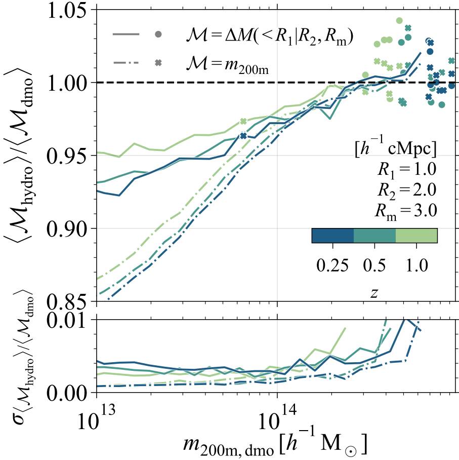
Figure 5.5: Top panel: The redshift dependence of the change in the aperture mass, \Delta \mathcal{M}_{\text{hydro}}(< 1 h^{-1} \text{cMpc} | R_2, R_m) (solid lines), and the 3D halo mass, m_{200\text{m}} (dash-dotted lines), stacked in bins of the 3D dark matter-only halo mass. All background correction annuli span the region between R_2 = 2 h^{-1} \text{cMpc} and R_m = 3 h^{-1} \text{cMpc} . Coloured lines show the different redshifts and crosses the halo mass for which r_{200\text{m,dmo}} = R_1 . Bins with fewer than 5 haloes show the individual results. The mass reduction decreases with increasing redshift at fixed 3D halo mass. At all redshifts, the aperture mass changes less than the 3D halo mass for m_{200\text{m,dmo}} \lesssim 10^{14} h^{-1} M_{\odot} . Bottom panel: The 1\sigma bootstrapped uncertainty in the mass change of hydrodynamical haloes compared to their matched DMO counterparts for the different mass measurements. The uncertainty in the mass reduction only increases for the rarest, high-mass haloes at higher redshift.
