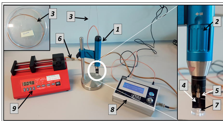
Figure 1. Digitally controlled hollow microneedle injection system to perform automated micro-injections into skin at a predetermined depth. Microneedle applicator ( 1 ); micrometer actuator ( 2 ); capillary ( 3 ); hollow microneedle ( 4 ); CapTite™ connectors ( 5 , 6 ); supporting plateau ( 7 ); applicator controller unit ( 8 ); syringe pump ( 9 ). See main text for explanation.
