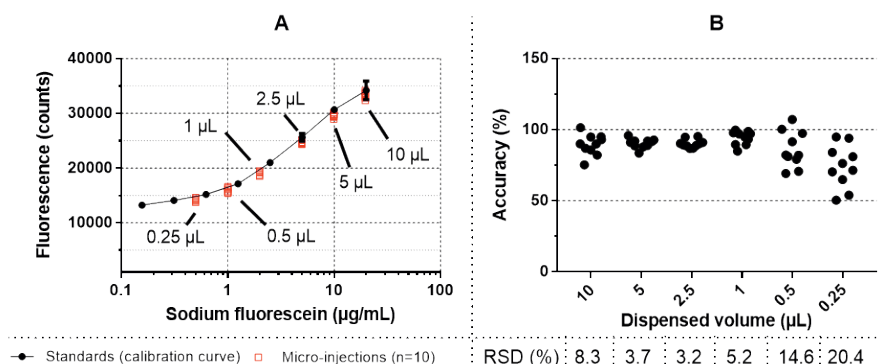
Figure 3. Digitally controlled micro-injections. Different digitally controlled volumes of a 1 mg/mL sodium fluorescein solution, ranging from 0.25–10 \mu\text{L} , were injected into 500 \mu\text{L} PBS and the fluorescence of the resulting solution was plotted against the corresponding fluorescein concentration. As a control, the fluorescence of fluorescein solutions with a known concentration was determined ( n=2 ) (A). The accuracy and precision of different digitally controlled micro-injections (B). Each digitally controlled volume was injected 10 times in 500 \mu\text{L} PBS. Abbreviation: relative standard deviation (RSD).
