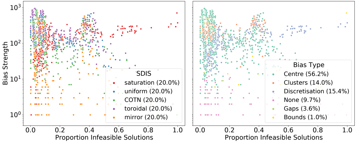
Figure 2: Bias Strength versus the fraction of infeasible solutions for all 1 620 configurations. Colours on the left plot indicate the boundary correction strategy (i.e. SDIS) and on the right the predicted type of SB using the BIAS toolbox.
