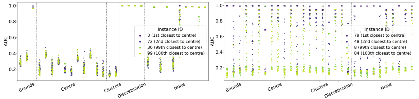
Figure 5: Performance results (AUC) for f_5 and f_{22} instances of the BBOB suite with 25 runs per configuration. Configurations are grouped by bias type on the X-axis. The instances with an optimum closest to the centre are shown in blue and the instances with an optimum furthest from the centre are shown in green.
