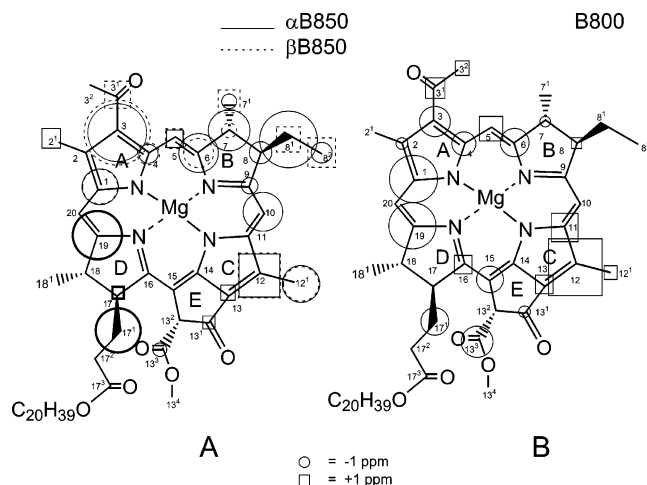
Figure 2. Estimated electronic shift changes ( |\Delta\delta| \geq 1.0 ppm), represented by circles (shielding effects) and squares (deshielding effects) for the \alpha B850 and the \beta B850 (A) and the B800 (B) cofactors in the LH2 complex. The size of the mark is proportional to the magnitude of \Delta\delta .
