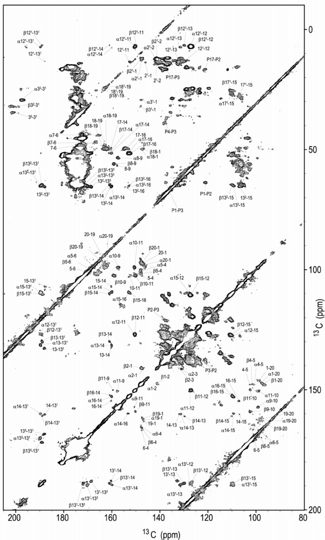
Figure 1. Contour plot of a high-resolution MAS 2D ^{13}\text{C} – ^{13}\text{C} RFDR solid-state NMR spectrum of the [\text{U-}^{13}\text{C}, ^{15}\text{N}] LH2 complex isolated from Rps. acidophila strain 10050. The data were obtained at 223 K with a spinning frequency of 13 kHz and a RFDR mixing time of 2.5 ms. The chemical shift correlation networks of the B800, the \alpha\text{B850} , and the \beta\text{B850} are indicated using the IUPAC numbering shown in Figure 2. \alpha\text{B850} and \beta\text{B850} are indicated by \alpha and \beta , respectively.
