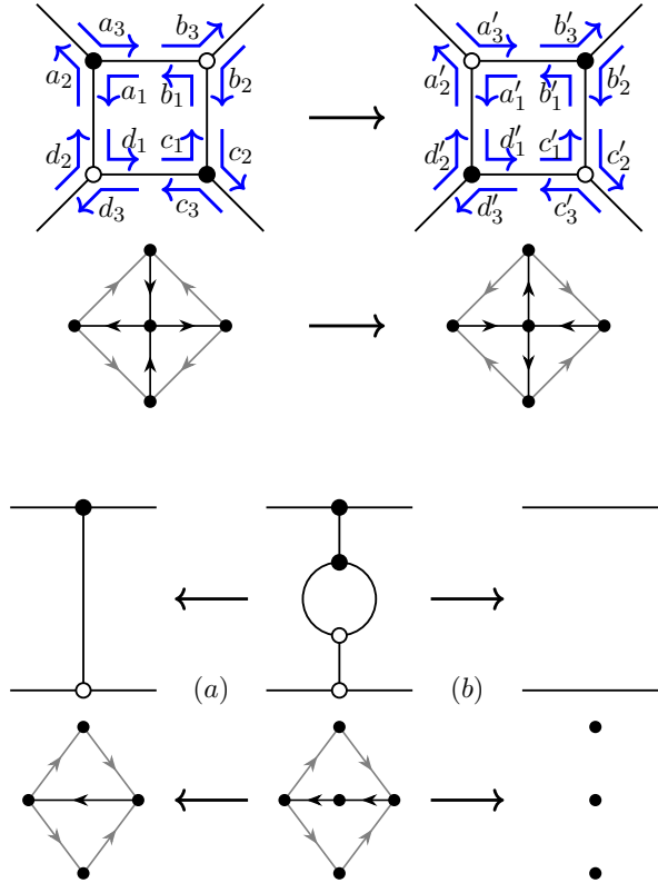
Figure 3.5. Top: change of bipartite graph under the spider-move and changes in the quiver. Grey arrows are for the entries \pm 1/2 of exchange matrix \epsilon . Bottom: two ways for parallel bigon reduction and changes in the quiver.
