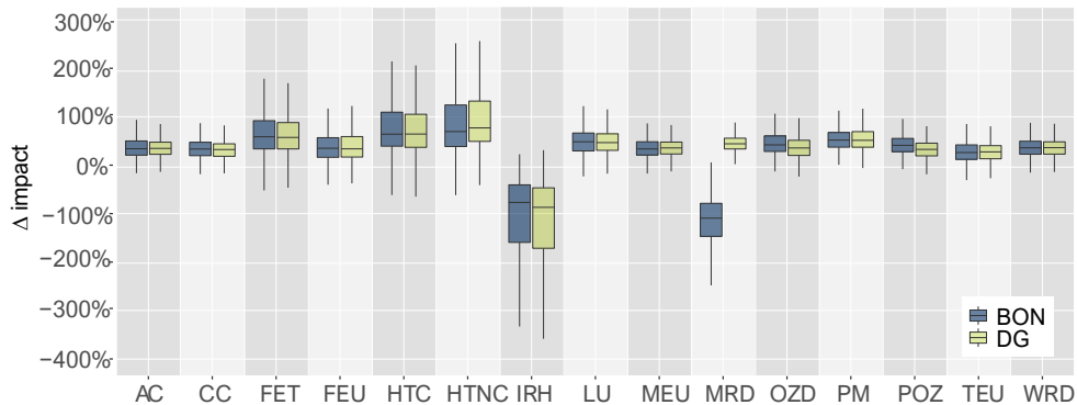
Figure 3-5 Monte Carlo simulation results for comparative impacts of III-V/Si PV systems vs. the reference single-Si PV system. Values are normalized to the deterministic impact score of the reference single-Si PV system. Positive values indicate a better performance of the III-V/Si systems. The middle line shows the median; the bottom and top edges of the box indicate the 25th and 75th percentiles respectively. The whiskers show minimum and maximum values, with outlier points removed.
