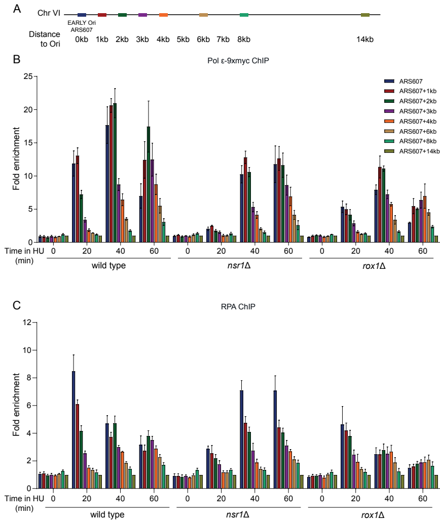
Figure 5. Polymerase \epsilon and RPA profiles at ARS607.
