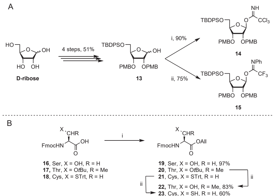
Scheme 2. A) Synthesis of ribosyl donors 14 and 15 . Reagents and conditions i) \text{Cl}_3\text{CCN} , DBU, acetonitrile. ii) \text{Cl}(\text{C}=\text{NPh})\text{CF}_3 , \text{Cs}_2\text{CO}_3 , acetone. B) Synthesis of amino acid acceptors 19 , 22 and 23 . Reagents and conditions: i) Allyl-Br, DIPEA, DMF. ii) TFA, DCM.
