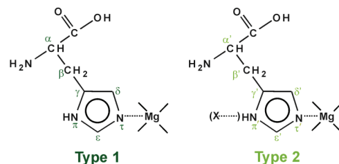
Figure 3. Schematic representation of DFT models of the type-1 and type-2 BChl–His neutral complexes without and with H-bonding at the \pi nitrogen, respectively. The total imidazole ring charge of the type-1 and type-2 histidines are calculated to be +0.10 and +0.19, respectively. The \tau -nitrogen–Mg distance is shortened by 0.03 Å in the presence of the H-bond at the \pi nitrogen.
