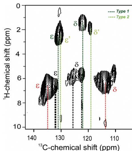
Figure 2. Contour plot sections of a 2D ^1\text{H} – ^{13}\text{C} heteronuclear dipolar correlation spectrum of [^{13}\text{C},^{15}\text{N}] -His-labeled bacterial RCs of R. sphaeroides collected at a magnetic field strength of 17.6 T. The cross-peaks from ^1\text{H} and ^{13}\text{C} at the \delta and \epsilon positions of axial histidines are shown in green. The significant ring-current effects on the axial histidines caused separation of their cross-peaks from those of nonaxial histidines in the RC. Two types of axial histidines, type 1 (dark-green) and type 2 (light-green) were detected.
