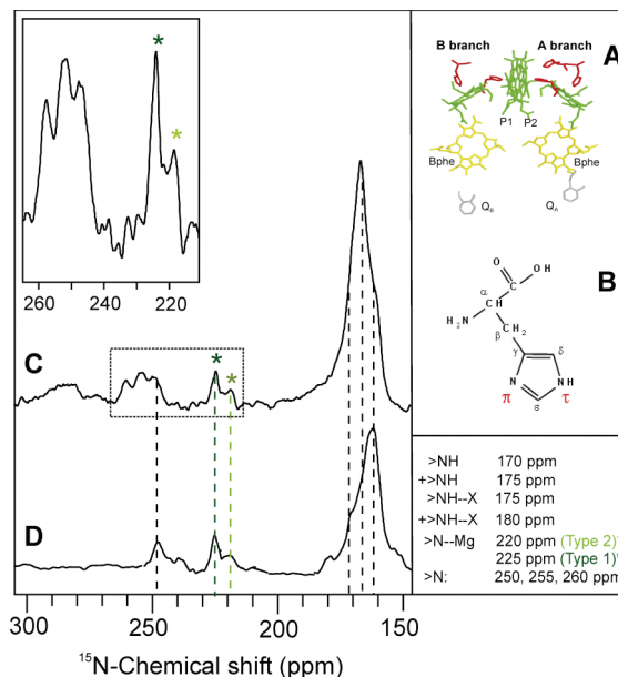
Figure 1. (A) Arrangement of cofactors in RCs of R. sphaeroides (R26). (B) Structure of His with nomenclature. (C, D) CP–MAS ^{15}\text{N} NMR spectra of (C) uniformly and (D) \tau - ^{15}\text{N} -His-labeled RCs measured in a magnetic field of 17.6 T at 220 K with a spinning frequency of 12 kHz. The data were collected in \sim 15\,000 scans with an acquisition time of 20 ms and a recycle time of 1 s. A detailed view of the region between 205 and 265 ppm is shown in the inset (upper left). Assignment of the ^{15}\text{N} peaks obtained from C and D is shown at the lower right. The asterisks indicate the positions of center-band signals from \tau nitrogens of axial histidines that interact with BChl a in the RC. The spectra reveal two different types of axial histidines, designated type 1 (dark-green dashed lines) and type 2 (light-green dashed lines), in bacterial RCs.
