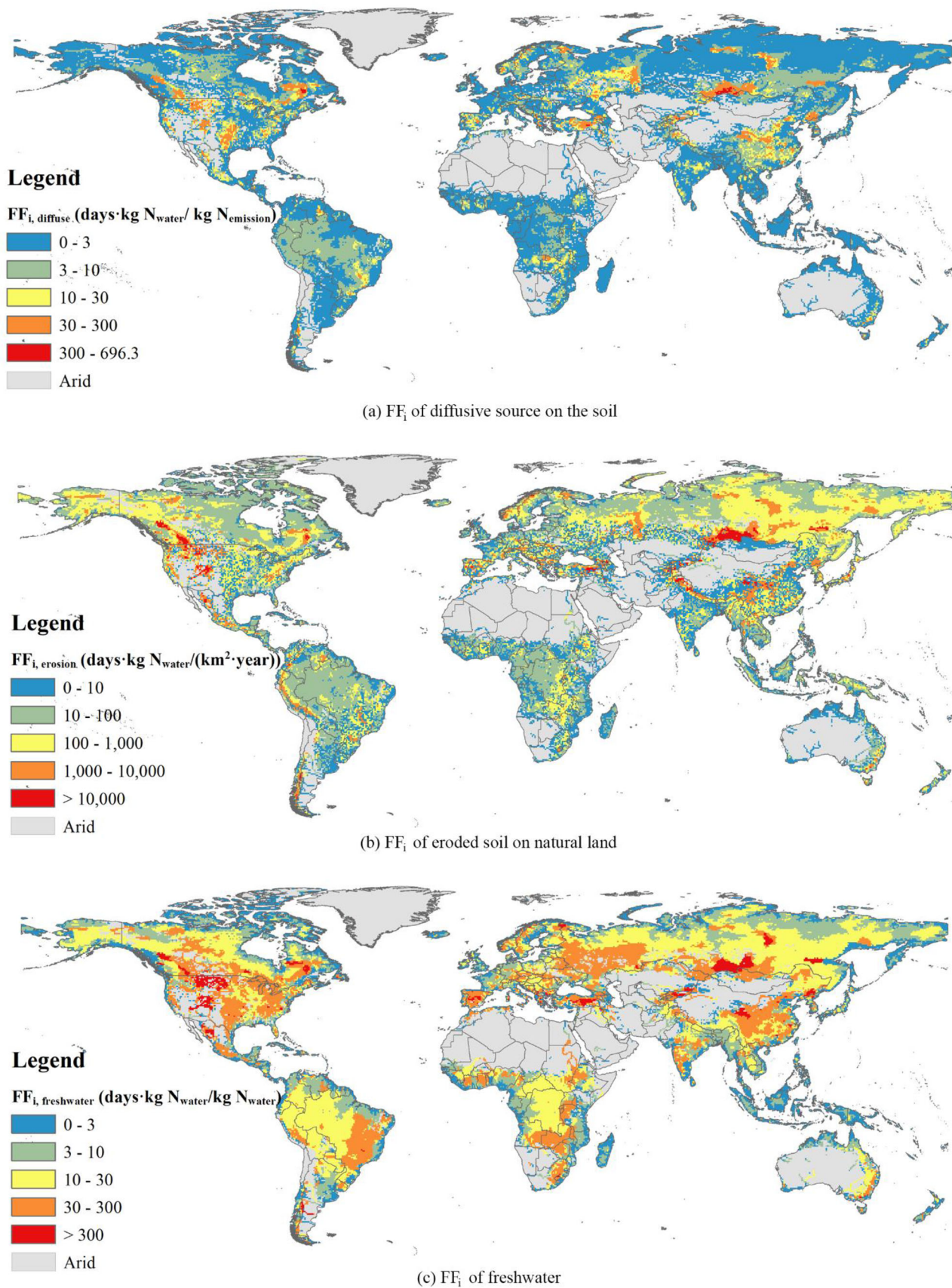
FIGURE 2 Cumulative FFs (fate factors) for N emission to freshwater for 0.5^\circ \times 0.5^\circ grid cells. (a) diffusive sources excluding erosion, (b) baseline erosion on natural land, and (c) direct emissions to freshwater, including point sources. For erosion, the difference of FFs between anthropogenic and natural erosion can be derived by multiplying with c_{\text{landuse}} - c_{\text{landuse}} for arable land and grassland are 45.30 and 2.41, respectively. The underlying data for this figure can be found in the Supporting Information
