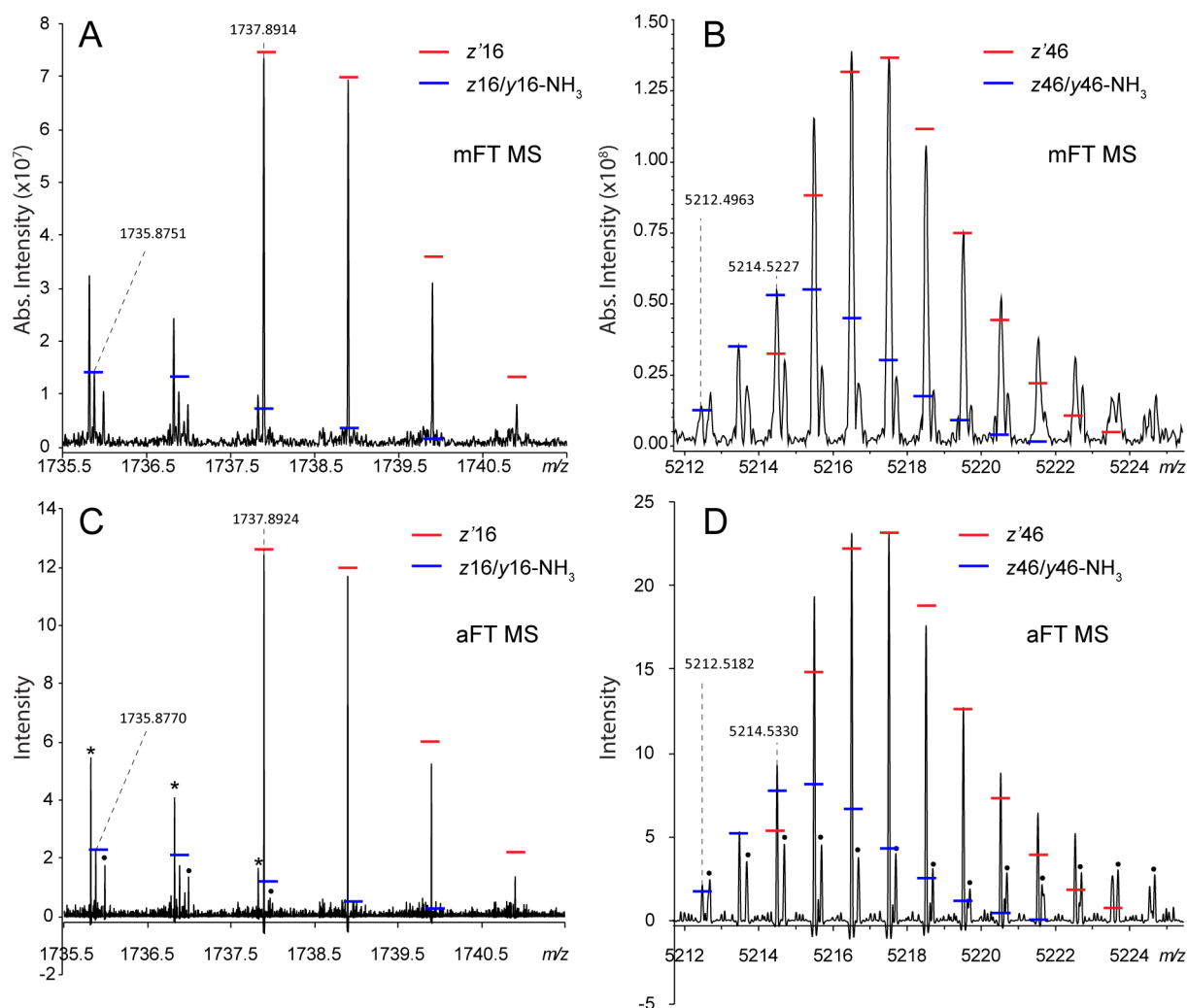
Figure 2. Isotopic distributions of z' and z/y - \text{NH}_3 ions detected in mFT (A and B) and aFT (C and D) MALDI-MS spectra of the heavy chain of NIST mAb. The colored marks indicate the expected intensities of the fragment ion isotopologues according to theoretical isotopic distributions of z/y - \text{NH}_3 (blue) and z' (red) ions. The theoretical m/z values of z'16 and z16/y16 - \text{NH}_3 are 1737.8919 and 1735.8762, respectively. The theoretical m/z -values of z'46 and z46/y46 - \text{NH}_3 of the mAb heavy chain are 5214.5200 and 5212.5044, respectively. The FoM values obtained for aFT isotopic distributions of z'16 and z'46 ions were 0.95 and 0.81, respectively. * b17 of NIST mAb light chain. • unidentified species.
