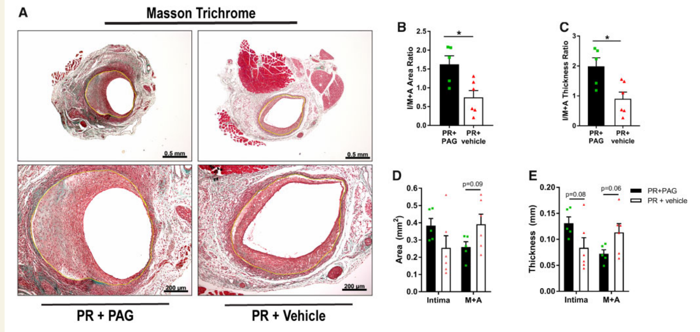
Figure 5 Cystathionine \gamma -lyase is required for protein restriction mediated attenuation of intimal hyperplasia. (A–D) Vein grafts assessments 28 days after surgery in PR-HFHC preconditioned LDLr^{-/-} mice injected with either vehicle or PAG during the one week preconditioning period prior to vein grafting; n = 5 –6/group. (A) Representative images of Masson trichrome-stained vein grafts; boundary between intimal (I) and medial + adventitial (M+A) layers is traced in yellow. Scale bars = 0.5 mm and 200 \mu m as indicated. (B and C) I/M+A area (B, 0.7 \pm 0.2 vs. 1.6 \pm 0.2 , P = 0.014 , Student's t -test) and thickness (C, 0.9 \pm 0.2 vs. 2.0 \pm 0.2 , P = 0.014 , Student's t -test) ratios. (D and E) Intimal and M+A area (D) and thickness (E); Student's t -test between \pm PAG treatment groups within layer. All data expressed as mean \pm SEM; * P < 0.05 .
