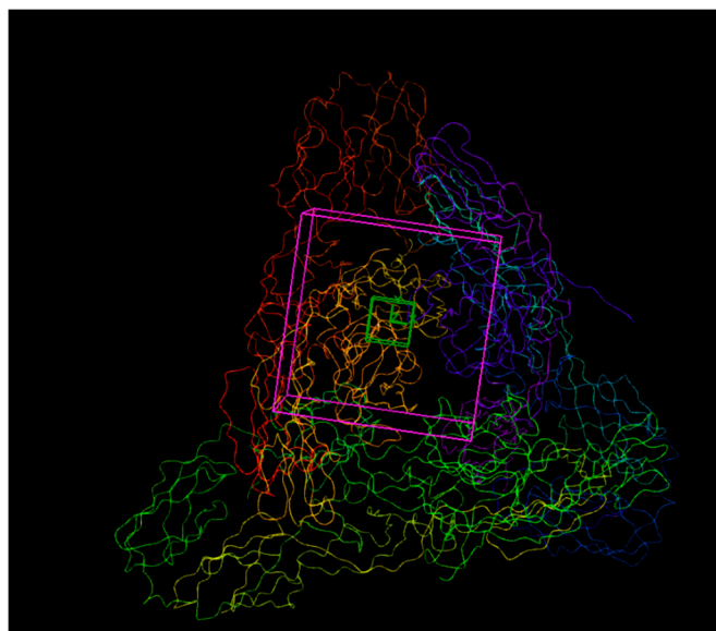
Figure A1. Docking grids used in molecular modeling of the trimeric complex of E1-E2 heterodimers. 36 Å docking grids (inner-box 10 Å and outer-box 46 Å) were prepared as described in the text of Appendix A.
