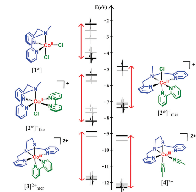
Fig. 6 Simplified energy level diagrams for [1^*] , [2^*]^+_{\text{fac}} , [2^*]^+_{\text{mer}} , [3]^{2+}_{\text{mer}} , and [4]^{2+} . Molecular orbital diagrams show only the five energy levels with the largest Co d-orbital contributions (highest-lying and lowest-lying energy levels are denoted in black, the remaining energy levels are denoted in grey). The three colours used in the structures indicate the fragments that were used in the DFT computations.
