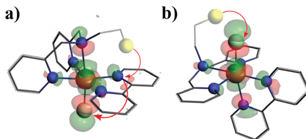
Fig. 7 Schematic drawings of the approach of the sulfur atom to replace chloride in (a) [2^*]^+_{\text{fac}} and (b) [2^*]^+_{\text{mer}} . The d_{z^2} character of [2^*]^+_{\text{fac}} and [2^*]^+_{\text{mer}} (SOMO–1 and SOMO, respectively) is shown as orbital lobes. The sulfur atom was omitted in the calculation of [2^*]^+_{\text{fac}} and [2^*]^+_{\text{mer}} , but is included for clarity.
