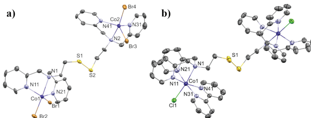
Fig. 4 Displacement ellipsoid plots (50% probability level) of (a) [\text{Co}_2(\text{L}^1\text{SSL}^1)(\text{Br})_4] ( [\mathbf{1}_{\text{Br}}] ) and (b) [\text{Co}_2(\text{L}^1\text{SSL}^1)(\text{bpy})_2(\text{Cl})_2]^{2+} ( [\mathbf{2}_{\text{Cl}}]^{2+} ) at 110(2) K. Hydrogen atoms, non-coordinated anions, and lattice solvent molecules are omitted for clarity.
