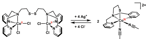
Scheme 1 Schematic representation of the reversible redox interconversion of the cobalt(II)-disulfide complex [\text{Co}_2(\text{L}^1\text{SSL}^1)\text{Cl}_4] ( [\mathbf{1}_{\text{Cl}}] ) and the cobalt(III)-thiolate complex [\text{Co}(\text{L}^1\text{S})(\text{MeCN})_2]^{2+} ( [\mathbf{4}]^{2+} ) induced by removal or addition of halide ions in MeCN solution. 13
