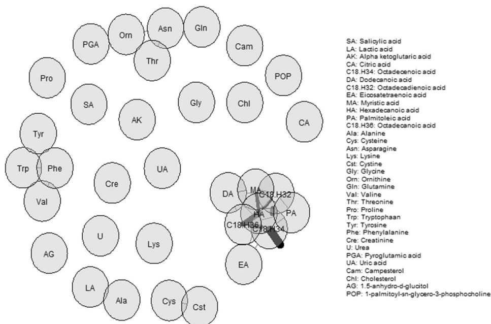
Fig. 1 Correlation network estimated using Pearson correlations. Each node represents one metabolite. The edges indicate the strength of the correlation. For this plot, only edges with an absolute weight of > 0.5 are shown
