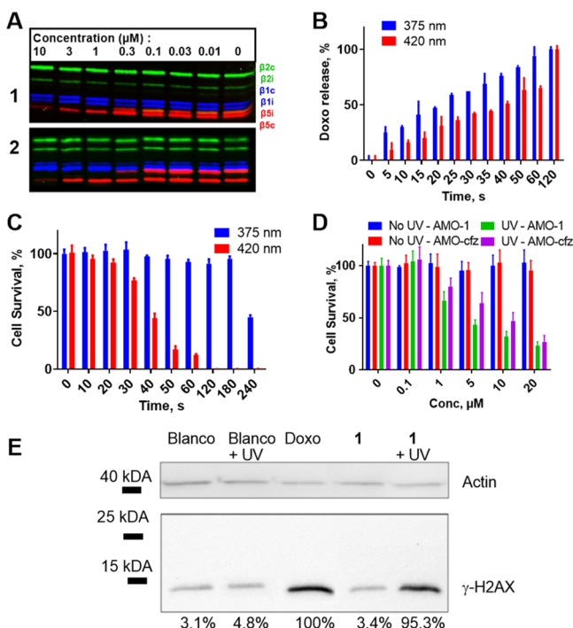
Figure 2. Biological evaluation of conjugates 1 and 2. (A) Competitive ABPP of compounds 1 and 2 with established proteasome subunit-selective activity based probes in AMO-1 cells. (B) Release of doxorubicin from 1 (10 \mu M) as determined by LC-MS. (C) Survival of AMO-1 cells after irradiation with 375 or 420 nm. (D) Cell survival of CFZ-resistant AMO-1 cells by treating with various concentrations of compound 1 and consequent irradiation with 375 nm for 60 s. (E) Western blot of \gamma -H2AX response after treatment of AMO-1 cells with 10 \mu M of compound followed with irradiation at 375 nm for 60 s.
