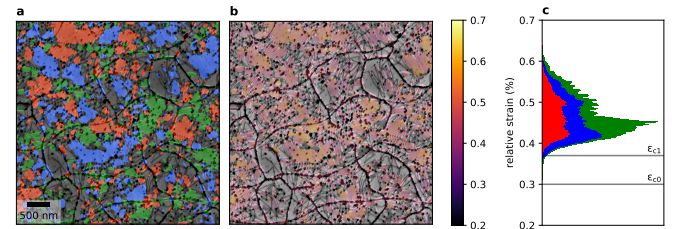
FIG. 8. a , Mask on sample A based on the GPA amplitudes labeling stripe domains in three directions in red, green and blue, showing stripe domains of several hundred nanometer across. b , Extracted strain for all three directions of stripe domains for a region in the sample A. c , Histogram of extracted strain values for the three stripe domain directions.
