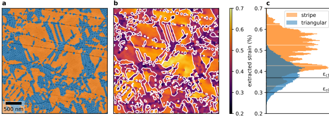
FIG. 7. a , Mask distinguishing stripe and triangular domains based on the triangle GPA magnitudes of sample B shown in Figure 6. Stripe domains are shown in orange, triangles in blue. b , Extracted strain for both types of domains in sample B for the same region. Boundary between the different domains is indicated with white lines. c , Histogram of extracted strain values for both phases.
