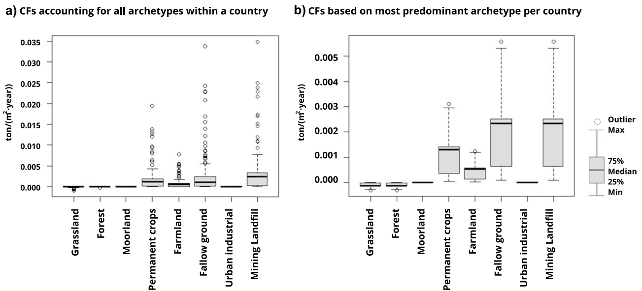
Fig. 2 Country-specific characterization factors for soil erosion potential impacts (in \text{ton}/(\text{m}^2\cdot\text{year}) )
