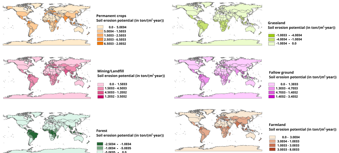
Fig. 3 Global maps of country-specific characterization factors for soil erosion potential impacts by land use occupation (in \text{ton}/(\text{m}^2\cdot\text{year}) )
