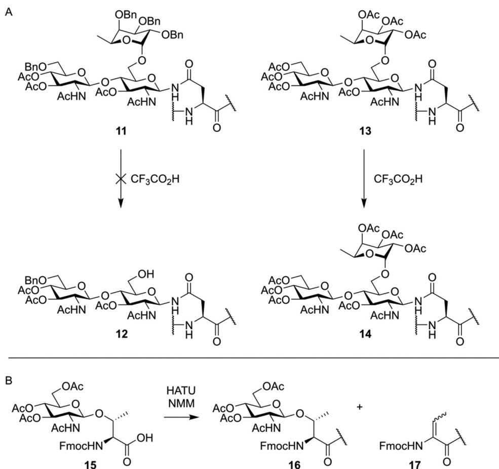
Fig. 3 (A) TFA mediated deglycosylation observed by Unverzagt and Kunz. 37 During TFA mediated deprotection of a peptide containing a trisaccharide (11) cleavage of the α-fucoside bond was observed yielding partially deprotected glycopeptide 12. A peptide containing an acetyl protected trisaccharide (13), when treated under similar conditions, did fully retain the fucose residue. (B) Base mediated β-elimination of an O-glycosylated threonine residue as observed by Zhang et al. 40
