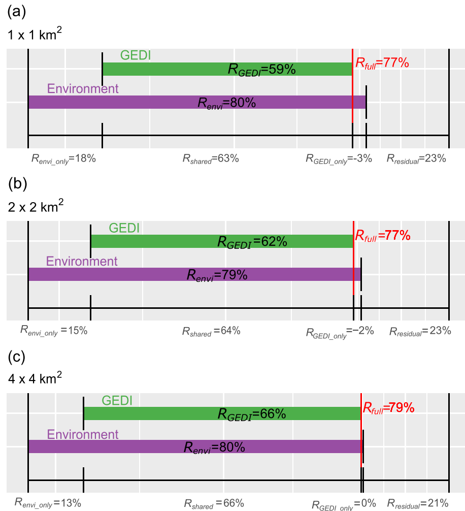
Figure 4. Variance of tree species richness explained by the GEDI variables (green, model 3), the environmental predictors (purple, model 2), and the full model with both GEDI and environmental predictors (red vertical line, model 4). Panels (a)–(c) show results from RF models using GEDI variables from 1 km 2 , 4 km 2 , and 16 km 2 buffer zones respectively. At the 16 km 2 buffer zone (c): GEDI canopy structure alone explains 66% of variation in tree species richness, 80% of the variation can be explained with environmental variables alone. The full model, combining all variables, explains slightly less (negative percentage on x-axis) of the variation: 79% (red line, panel c); hence resulting in 21% unexplained variation.
