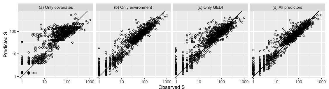
Figure 3. Observed versus predicted plots of the response variable of the random forest (RF) models with the 16 km 2 buffer zone for the four models. Diagonal line shows the perfect 1:1 match.
