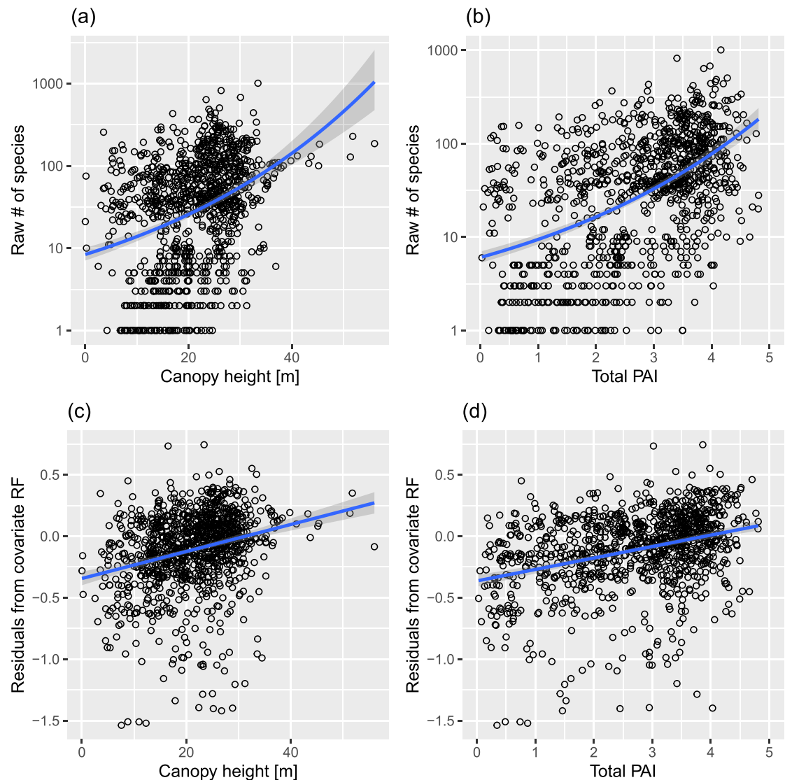
Figure 2. Bivariate relationships between number of species (species richness, S ) in forest plots and two GEDI-derived variables: canopy height (a), (c) and total Plant Area Index—PAI (b) and (d). In the top row (a) and (b) are raw species numbers as reported in each study, and a quasi-Poisson regression (log link function). In the bottom row (c) and (d) we show residuals of a random forest model accounting for plot area, number of tree individuals, and minimum diameter at breast height. To calculate the residuals, we \log_{10} -transformed the observed and predicted values of S . A linear regression (normal errors) was then fitted to the residuals. All relationships are statistically significant (with P < 0.001 ). Grey bands show standard errors.
