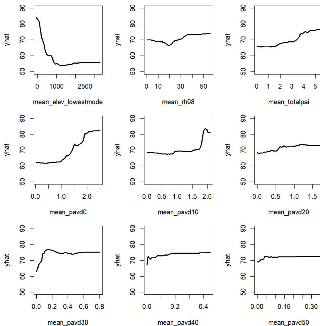
Figure D1. Partial dependence plots for random forest with covariates and GEDI predictors only (derived at 4 \times 4 km buffer zone around each forest plot). Yhat is the response of species richness to a given predictor, after accounting for effects of other predictors and covariates. Abbreviations: mean_elev_lowestmode is the ground elevation, mean_rh98m is Canopy Height (RH98), mean_totalpai is Total Plant Area Index (PAI), mean_pavd0—mean_pavd50 is the total PAI at 10 m vertical intervals, with pavd0 meaning total PAI between 0–10 m vertically, pavd10 referring to total PAI between 10–20 m, etc.
