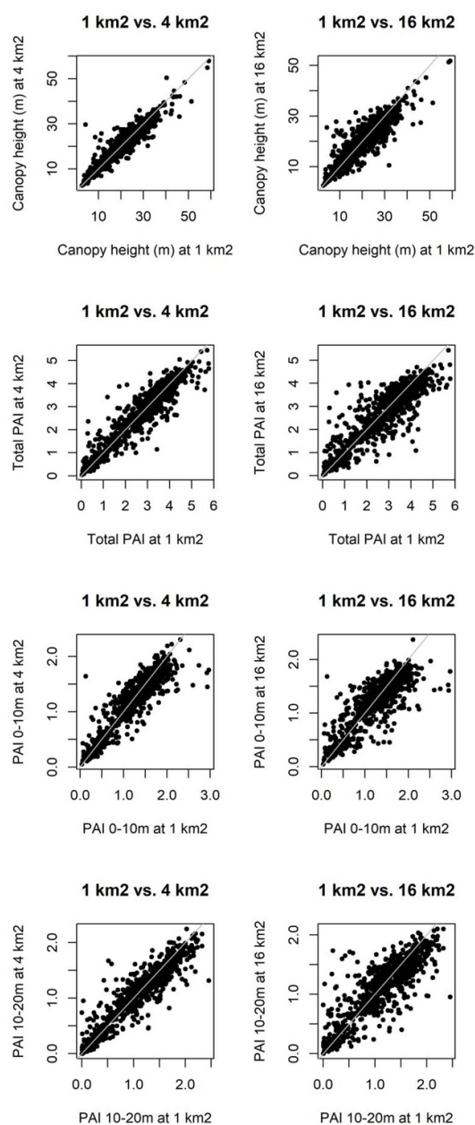
Figure C1. Relation between canopy structure metrics of GEDI at the 1 km 2 vs. 4 km 2 buffer zones and the 1 km 2 vs. 16 km 2 buffer zones.
