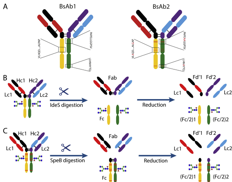
Fig. 1. A) Comparison of amino acid differences between BsAb1 and BsAb2. Exchanged amino acids are shown in red. Glycans are removed for simplicity. Hinge region cleavage and reduction of BsAbs leading to six different subunits. B) IdeS digestion and reduction of BsAb1. C) SpeB cleavage and reduction of BsAb2. Red stripes in the Fc indicate LALA PG mutation. (For interpretation of the references to color in this figure legend, the reader is referred to the Web version of this article.)
