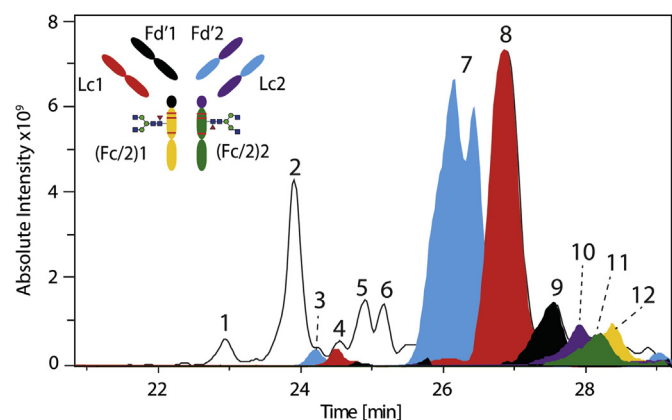
Fig. 5. BPE (black trace) and EIEs (color fill) for all the six subunits (7–12, compare Table S4) of BsAb2 obtained by sheathless CE-FT-ICR-MS after SpeB cleavage and DTT reduction. Truncated versions of BsAb2 are numbered from 1–6 (compare Table S5). BGE: 20% Acetic acid containing 10% MeOH. EIEs: Peak 7 ( 1012.15 + 1060.11 + 1113.12 \pm 0.1 m/z); Peak 8 ( 1165.59 + 1116.86 + 1171.95 \pm 0.1 m/z); Peak 9 ( 1040.36 + 998.21 + 084.97 \pm 0.1 m/z); Peak 10 ( 917.61 + 950.83 + 986.08 \pm 0.1 m/z); Peak 11 ( 922.47 + 956.14 + 993.47 \pm 0.1 m/z); Peak 12 ( 1004.28 + 1044.41 + 967.16 \pm 0.1 m/z). (For interpretation of the references to color in this figure legend, the reader is referred to the Web version of this article.)
