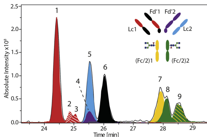
Fig. 3. BPE (black trace) and EIEs (color fill) for the six chains and proteoforms of BsAb1 obtained by sheathless CE-FT-ICR-MS after IdeS cleavage and DTT reduction (labelled from 1–8, compare Table 2). Peak number 9 contains both Fc/2 fragments as a complex. BGE: 20% Acetic acid containing 10% MeOH. EIEs: Peak 1 (1009.10+1057.06+1109.96±0.1 m/z ); Peak 2 (1009.78+1057.91+1110.70±0.1 m/z ); Peak 3 (999.50+1047.14+1099.50±0.1 m/z ); Peak 4 (1038.80+1082.04+1129.09±0.1 m/z ); Peak 5 (1066.94+1117.75+1173.49±0.1 m/z ); Peak 6 (1025.95+1065.41+1107.94±0.1 m/z ); Peak 7 (927.83+963.49+1001.95±0.1 m/z ); Peak 8 (938.26+974.26+1013.15±0.1 m/z ); Peak 9 (1398.96+1438.98+1481.22±0.1 m/z ). (For interpretation of the references to color in this figure legend, the reader is referred to the Web version of this article.)
