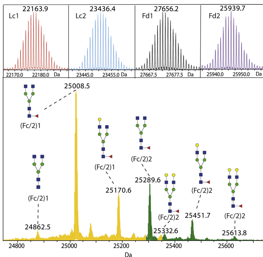
Fig. 4. Deconvoluted mass spectra of the Lc1 (red), Lc2 (blue), Fd1 (black) and Fd2 (purple) obtained after sheathless CE-FT-ICR-MS of mAb1. Additional Fc/2 fragments ((Fc/2)1 in yellow and (Fc/2)2 in green) are shown with different glycoforms (G0, G0F, G1F, G2F). BGE: 20% Acetic acid containing 10% MeOH. (For interpretation of the references to color in this figure legend, the reader is referred to the Web version of this article.)
