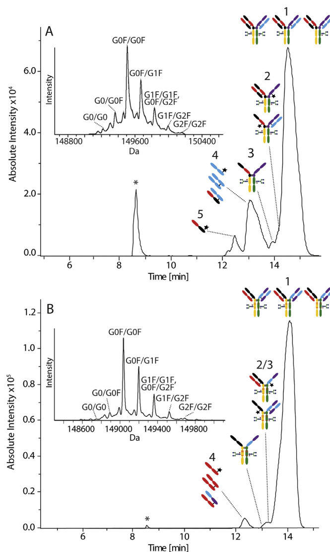
Fig. 2. Sheathless CE-qTOF-MS of intact BsAbs. A) Base peak electropherogram (BPE) of BsAb1 (labeled from 1 to 5, see Table 1) and deconvoluted spectrum of peak 1 (inset). B) Base peak electropherogram (BPE) of BsAb2 (labeled from 1 to 4, see Table S1) and deconvoluted spectrum of peak 1 (inset). BGE: 10% Acetic acid. (*) non-protein peak.
