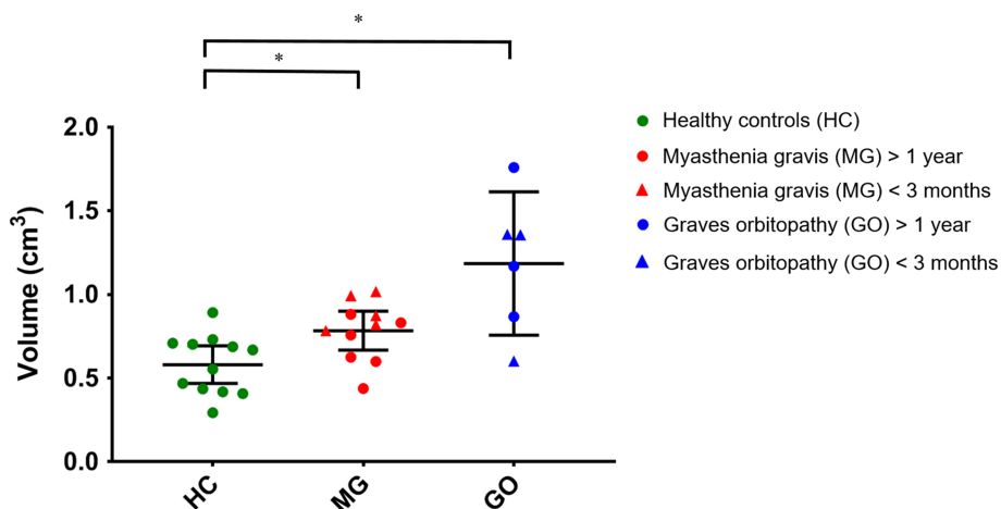
FIGURE 4 Mean muscle volumes of the four recti muscles per subject. Data are shown as mean and standard deviation for healthy controls (HC; green), myasthenia gravis (MG) (red) and Graves' orbitopathy (GO) patients (blue). The mean volume was 0.6 \pm 0.2 \text{ cm}^3 in HC, 0.8 \pm 0.2 \text{ cm}^3 in MG patients and 1.2 \pm 0.4 \text{ cm}^3 in GO patients. The MG and GO patients had significantly higher muscle volume compared with muscle controls ( P = .007 and P < .001 , respectively). Statistical significance is indicated by asterisks
