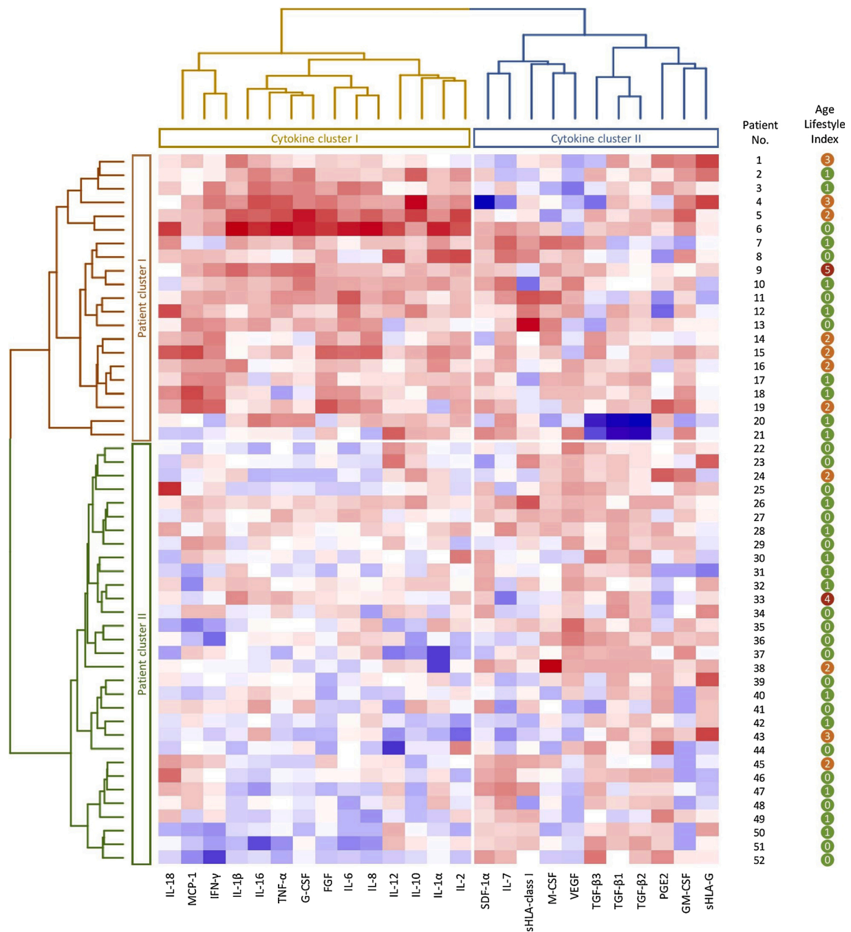
Fig. 2. Cluster analysis. Two-way hierarchical cluster analysis with Euclidean distance and Ward's aggregation method. Columns represent cytokines and other immunological factors present in the seminal plasma. Rows represent 52 patient samples (seminal plasma from male partners of women with unexplained RPL). Cytokine concentrations are indicated using a colour scale, ranging from blue (low) to red (high). Both patients and cytokines were separated by the algorithm into two main clusters, indicated as Patient clusters I and II and Cytokine clusters I and II. Patient cluster I contains patients that showed higher expression of pro-inflammatory factors in the seminal plasma compared to Patient cluster II. The Age Lifestyle Index (scoring method explained in paragraph Data analysis and statistics) for each patient is shown on the right, ranging from green (low) to red (high) (For interpretation of the references to colour in this figure legend, the reader is referred to the web version of this article.).
