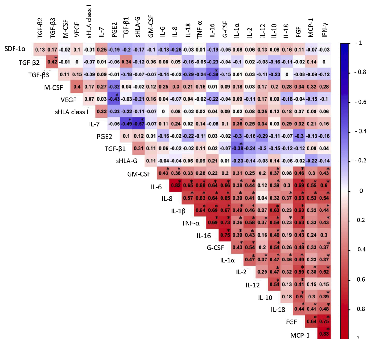
Fig. 1. Correlation matrix. Spearman's rank correlations ( \rho ) between individual seminal plasma signalling molecules. Red colour indicates a positive correlation, white colour indicates no correlation and blue colour indicates a negative correlation. *Benjamini-Hochberg adjusted P -value < 0.05 (For interpretation of the references to colour in this figure legend, the reader is referred to the web version of this article.).
