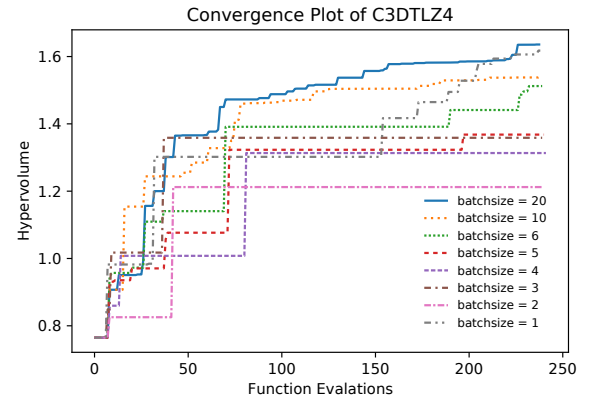
(d) Convergence plot for C3DTLZ4 function. With a different color for different batch sizes used in the acquisition function.
