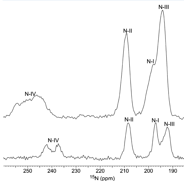
Figure 3. 1D CP/MAS 15 N spectrum for uniformly 13 C- and 15 N-enriched chlorosomes from the bchQR mutant (bottom trace) and WT (top trace) of C. tepidum recorded in a field of 17.6 T at a 12 kHz MAS frequency. The CP contact time was set to 5.12 ms; 86000 scans were collected with a recycle delay of 2 s.
