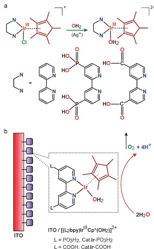
Figure 1. a) Cp * -Ir-derived complexes with bpy and L 2 bpy ligands; b) Schematic representation of the immobilized [(L 2 bpy)Ir III Cp * -(OH 2 )] 2+ (Cat.Ir-PO 3 H 2 and Cat.Ir-COOH for L = PO 3 H 2 and COOH, respectively) on ITO for electrochemical water oxidation. The metal-stabilizing Cp * ligand is highlighted in brown-red.
