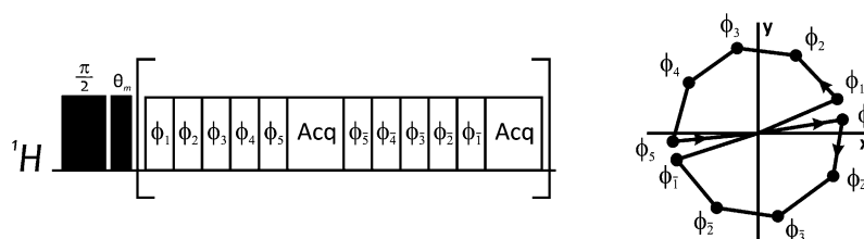
Figure 2. The wPMLG pulse sequence applied in this study (left panel) and corresponding rf pulse trajectories. Following excitation with a \pi/2 pulse and a pulse at the magic angle, a PMLG train of five pulses is applied, followed by an acquisition window. The phases of the rf pulses are alternated between the first and second halves of the PMLG scheme, according to \Phi_1=20.78^\circ , \Phi_2=62.35^\circ , \Phi_3=103.92^\circ , \Phi_4=145.49^\circ , \Phi_5=187.06^\circ , \Phi_6=7.06^\circ , \Phi_7=325.49^\circ , \Phi_8=283.92^\circ , \Phi_9=242.35^\circ , \Phi_{10}=200.78^\circ to provide the trajectory of the rf pulses during the wPMLG experiment according to the right panel.
