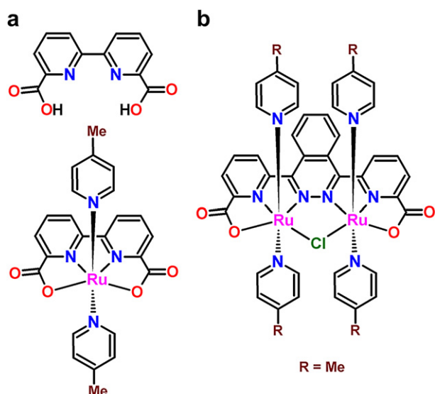
Fig. 5 – (a) A H_2dcabpy ligand derived mono-site [Ru^{II}(H_2dcabpy)(pic)] complex, ( H_2dcabpy is 2,2'-bipyridine-6,6'-dicarboxylic acid; pic is 4-picoline) and (b) a dinucleating dicarboxylic modified ligand bis(capyptz) based dimeric ruthenium catalyst [Ru_2(biscapyptz)] ( bis(capyptz) = 1,4-bis(6'-COOH-pyrid-2'-yl)phthalazine ) [55,56].
