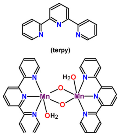
Fig. 2 – 2,2':6',2''-terpyridine (terpy) derived di- \mu -oxo di-terpy dimanganese diaquo water oxidation complex, [(terpy)(H_2O)Mn^{III}(\mu-O)_2Mn^{IV}(terpy)(H_2O)]^{3+} (Mn dimer).
