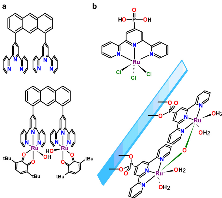
Fig. 8 – (a) A bis(ruthenium–hydroxo) complex, bearing a novel bridging type ligand 1,8-bis(2,2':6',2''-terpyridyl)anthracene (btpyan) and (b) a surface anchored terpy-Ru dimer [(PO 3 H 2 -terpy)(H 2 O) 2 Ru III ( \mu -O)Ru III (H 2 O) 2 (PO 3 H 2 -terpy)] 4+ (PO 3 H 2 -terpy = 4'-phosphonato-2,2':6',2''-terpyridine) for electrocatalytic water oxidation.
