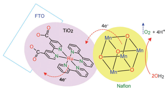
Figure 8. Schematic of a light-driven photoelectrochemical assembly with a tetramanganese ( 2\text{Mn}^{\text{III}}-2\text{Mn}^{\text{IV}} )-cubane catalyst. The Mn-cubane complex is impregnated into a Nafion membrane supported on a [\text{Ru}^{\text{I}}(\text{bpy})_2(\text{COO})_2^-] light sensitizer on \text{TiO}_2 film. FTO = fluorine tin oxide.
