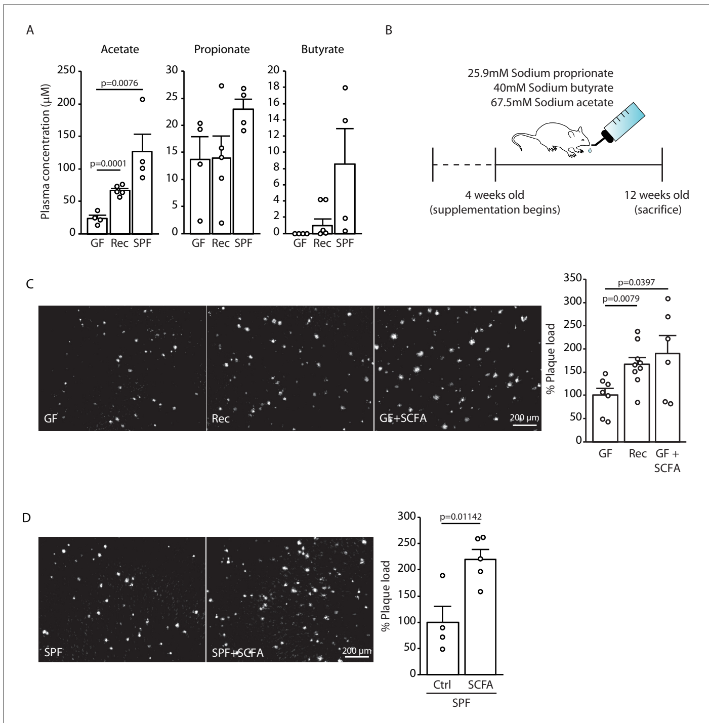
Figure 2. Short chain fatty acids (SCFA) are mediators of A \beta plaque deposition. (A) Plasma SCFA concentrations of acetate, butyrate, and propionate were quantified using GC/MS-based metabolomics analysis, showing an increase in specific pathogen-free (SPF) compared to germ-free (GF) mice (ANOVA; n(\text{GF}) = 4 , n(\text{Rec}) = 5 , n(\text{SPF}) = 4 ; two individual experiments). (B) Experimental plan for SCFA supplementation in GF mice. Four weeks old GF mice have been treated with SCFA in drinking water for 8 weeks. (C) Representative images from GF (control-treatment), Rec, and GF supplemented with SCFA mice showing a significant increase in A \beta plaque load upon SCFA administration (ANOVA; n(\text{GF}) = 7 , n(\text{Rec}) = 9 , n(\text{GF} + \text{SCFA}) = 6 ; three individual experiments). (D) SPF APPPS1 mice were supplemented with control or SCFA in drinking water for 4 weeks (from 8 to 12 weeks of age). Histological analysis revealed a significantly increased plaque load in SCFA-supplemented SPF mice compared to control treatment (unpaired T-test; n(\text{Ctrl}) = 4 , n(\text{SCFA}) = 5 ; one individual experiment). All data in this figure are presented as mean \pm SEM.
