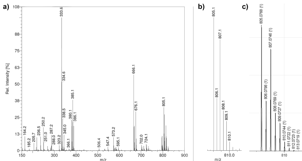
Figure AIV.11. ESI-MS spectrum of compound a) [3\text{Cl}] dissolved in methanol; b) the experimental isotopic distribution; c) simulated isotopic distribution at m/z 800–815. ESI-MS found (calcd.) for [3\text{Cl} - 2\text{Cl}^- + \text{HCOO}^-]^+ m/z 805.1 (805.08), for [3\text{Cl} - 3\text{Cl}^- + \text{HCOO}^-]^{2+} m/z 385.1 (385.1), and for [3\text{Cl} - 2\text{Cl}^-]^{2+} m/z 380.1 (380.04).
