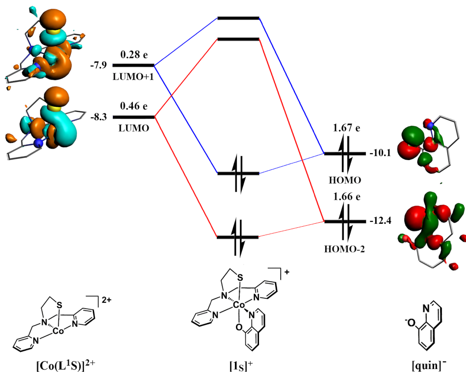
Figure AII.20. Molecular orbital diagram for the interaction between the fragments [\text{Co}(\text{L}^1\text{S})]^{2+} and [\text{quin}]^- in [1\text{s}]^+ . Fragment molecular orbital energies (in eV) obtained from the Kohn-Sham Fock matrix diagonal elements (see references 1-3 for details).
