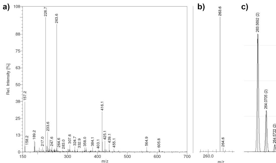
Figure AL.9. ESI-MS spectrum of a) the isolated brown-reddish powder from the reaction between [2\text{Cl}](\text{BPh}_4)_2 with \text{AgSbF}_6 , the powder was dissolved in acetonitrile; b) the experimental isotopic distribution; c) simulated isotopic distribution. ESI-MS found (calcd.) for [(\text{Co}(\text{bpy})_3)_2]^+ m/z 263.6 (263.6).
