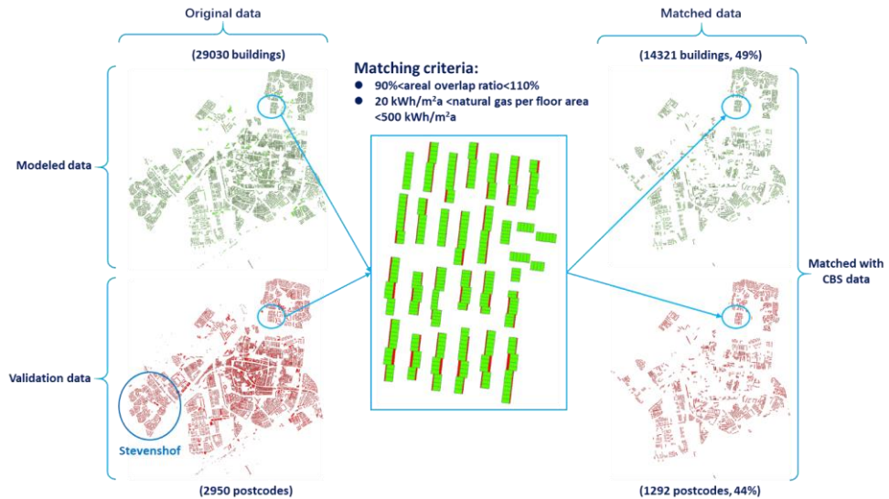
Figure 2.2 Mapping the modeled results with measured data from CBS. The green polygons are BAG buildings and the red are the CBS buildings dissolved by postcode. The natural gas consumption is expressed in kWh/m 2 a. In Stevenshof, the buildings are connected to district heating networks, so it is filtered.
