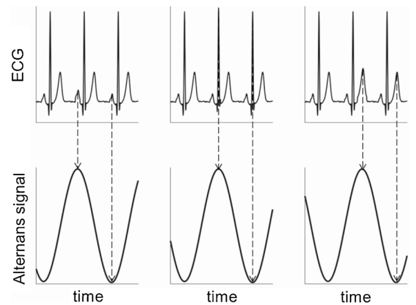
Fig. 4. Qualitative representation of the electrocardiogram (ECG, first row) and corresponding alternans signal (second row) at the output of the enhanced adaptive matched filter (EAMF) in case of P-wave alternans (PWA; first column), QRS-complex alternans (QRSA; second column) and T-wave alternans (TWA; third column). In all cases the alternans signal is a pseudo-sinusoid. However, the pseudo-sinusoid phase depends on the alternans kind: in case of PWA, pseudo-sinusoid maxima and minima fall in correspondence of the P wave; in case of QRSA, pseudo-sinusoid maxima and minima fall in correspondence of the QRS complex; and in case of TWA, pseudo-sinusoid maxima and minima fall in correspondence of the T wave.
