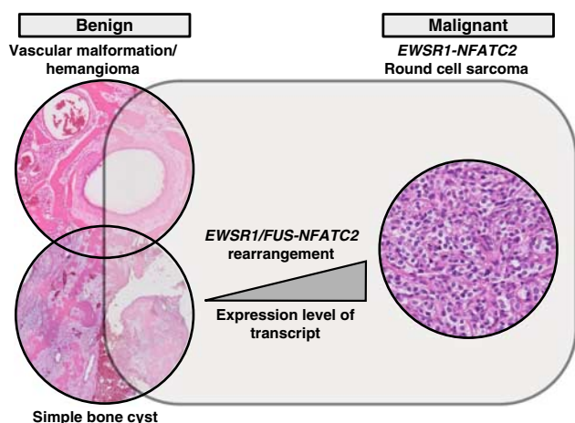
FIGURE 7. A proposed genetic relationship between EWSR1-NFATC2 translocation carrying vascular malformation/hemangioma, SBC and round cell sarcomas. All entities carry the same genetic rearrangement but as EWSR1-NFATC2 round cell sarcomas has amplification of the translocated genes an increased expression of the fusion transcript may contribute to the malignant behavior.
